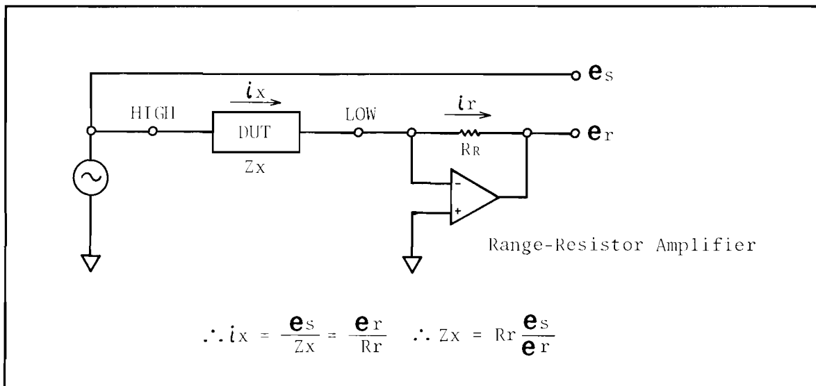
Figure 8-5. Current-To-Voltage Conversion Method
