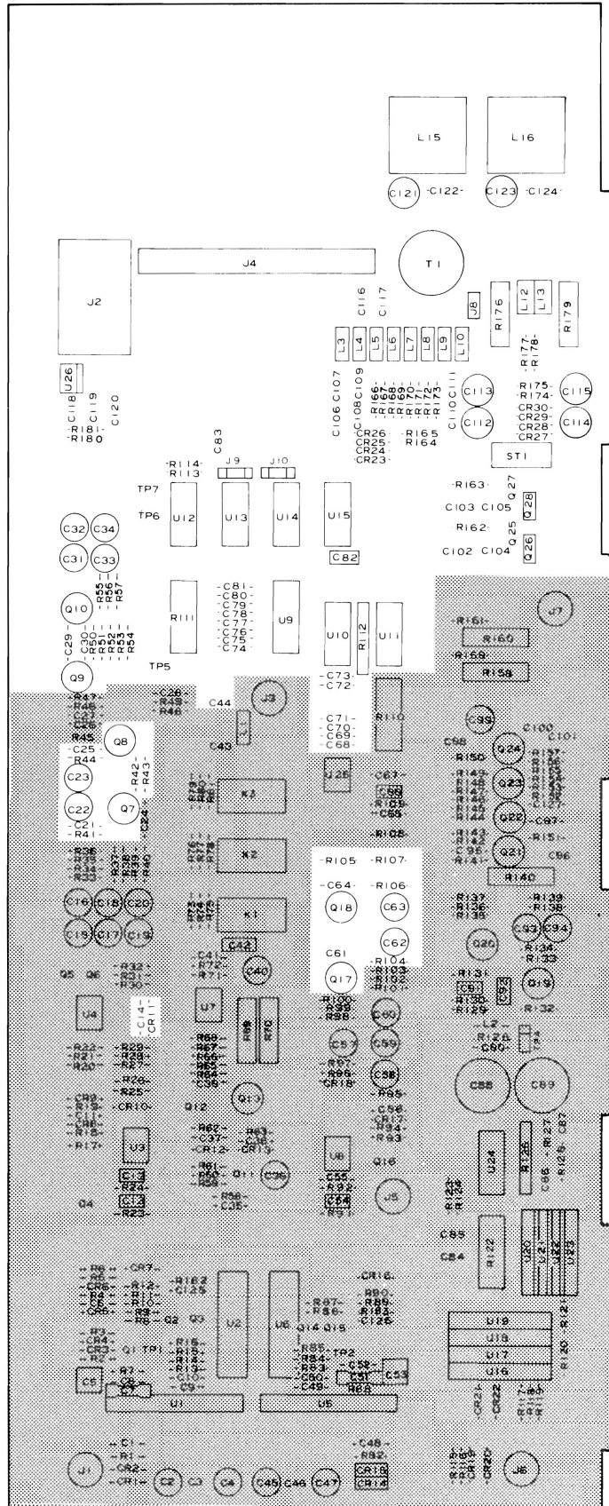
A20 Range Resistor Component Locations (2 of 2) 8-125
