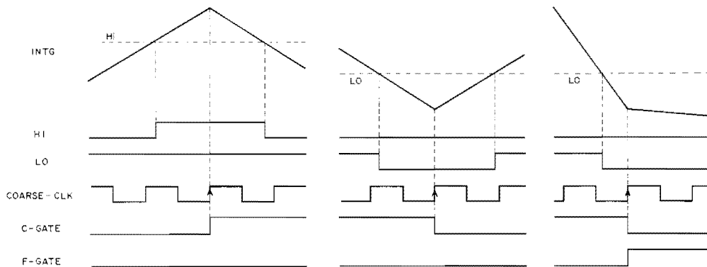
Figure A9-4. A-D Converter Timing Diagram
