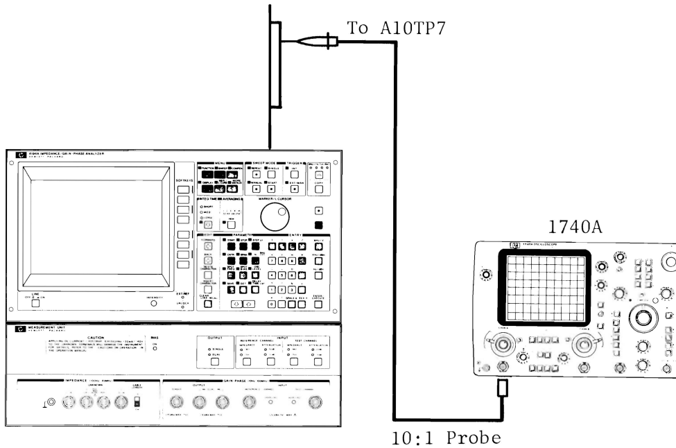
Figure 5-10. IF Level Adjustment Setup
