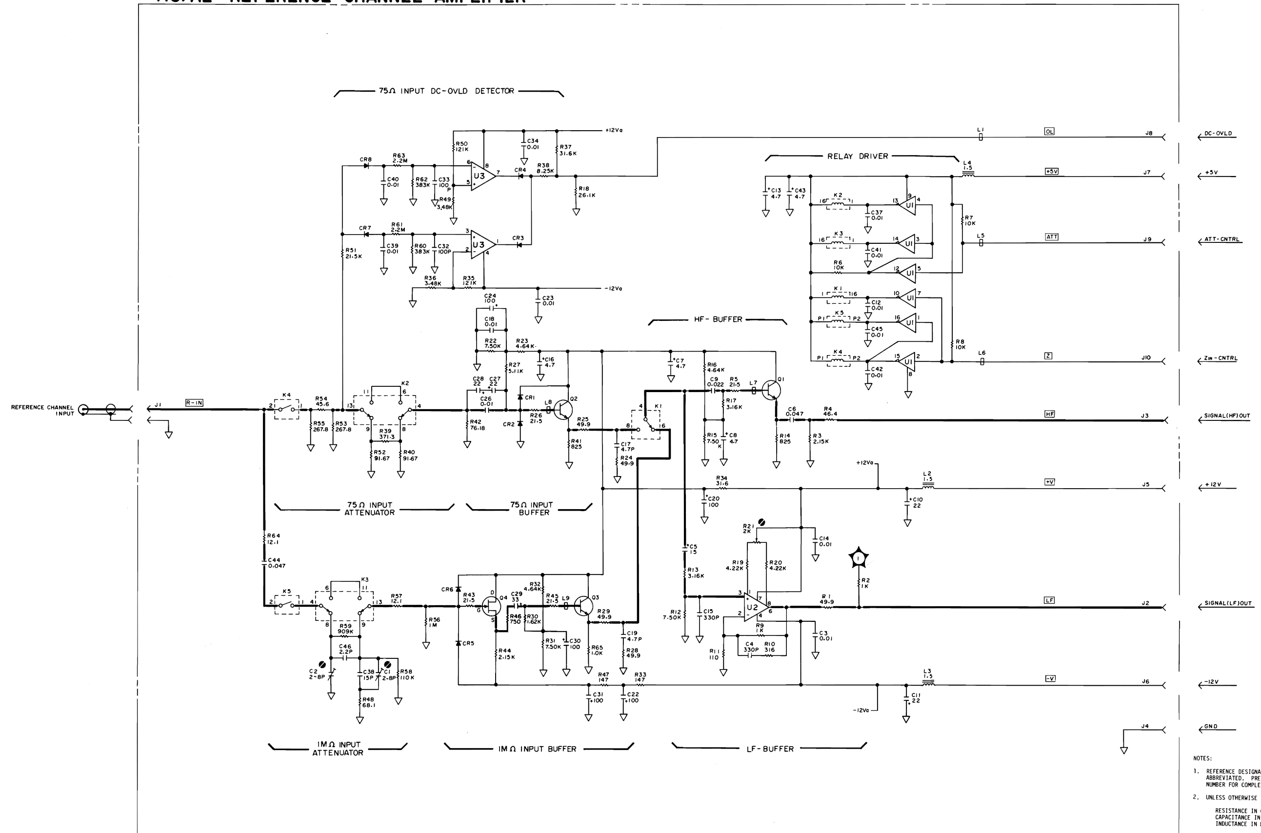
A31A2 Reference Channel Amplifier Schematic Diagram
