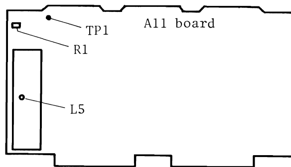
Figure 5-12. VCO Center Frequency Adjustment Locations
