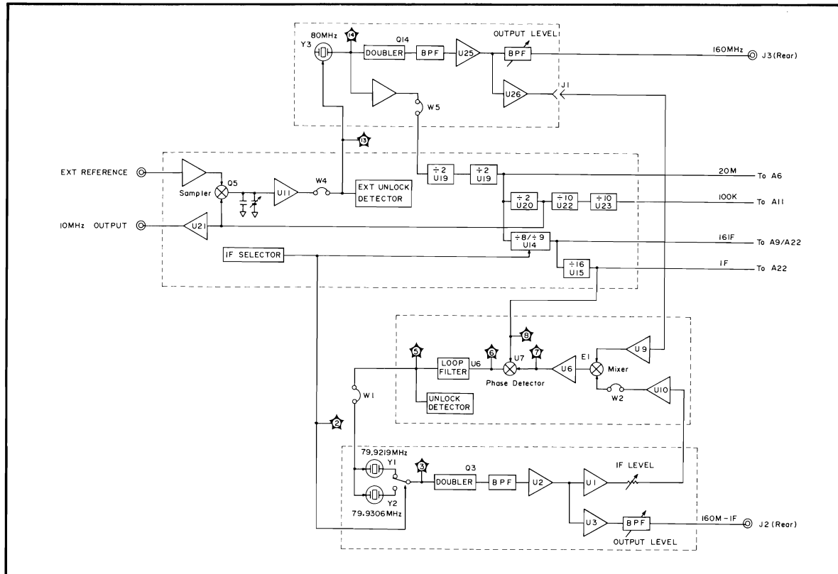
Figure A10-1. A10 Board Block Diagram
