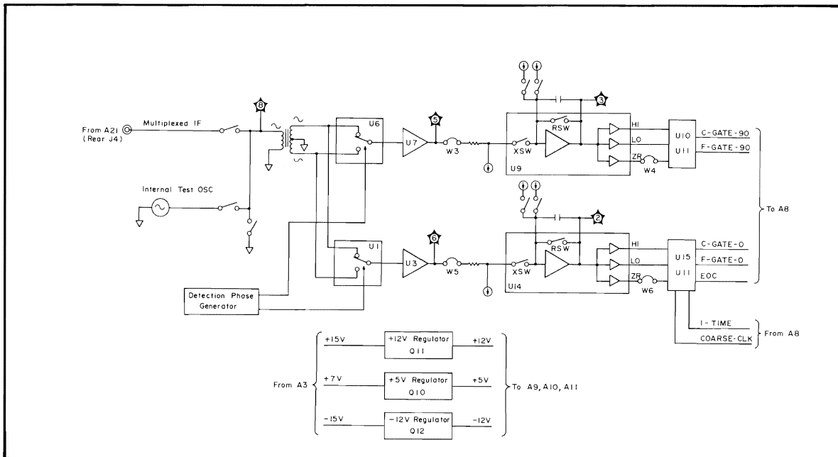
Figure A9-1. A9 Board Block Diagram
