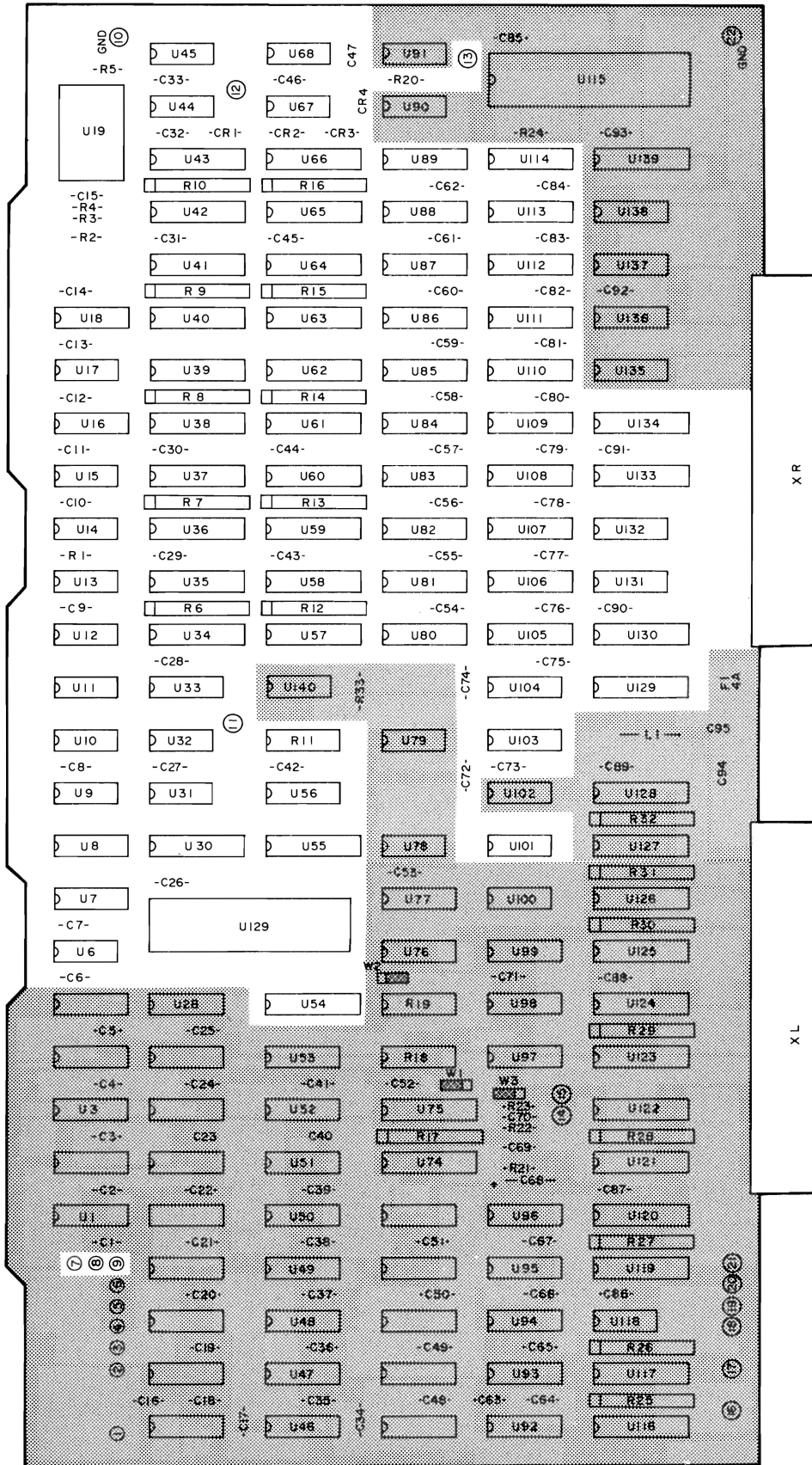
A7 GDC/RAM Component Locations (2 of 2)
