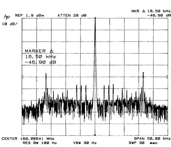
Figure 5-18. Incorrectly Adjustment API 3 Spectrum
