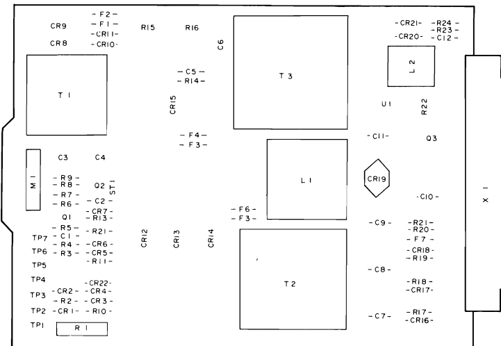
A3 Power Supply Output Component Locations
