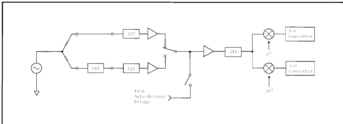
Figure 8-12. Gain-Phase Measurement Circuit Simplified Block Diagram
