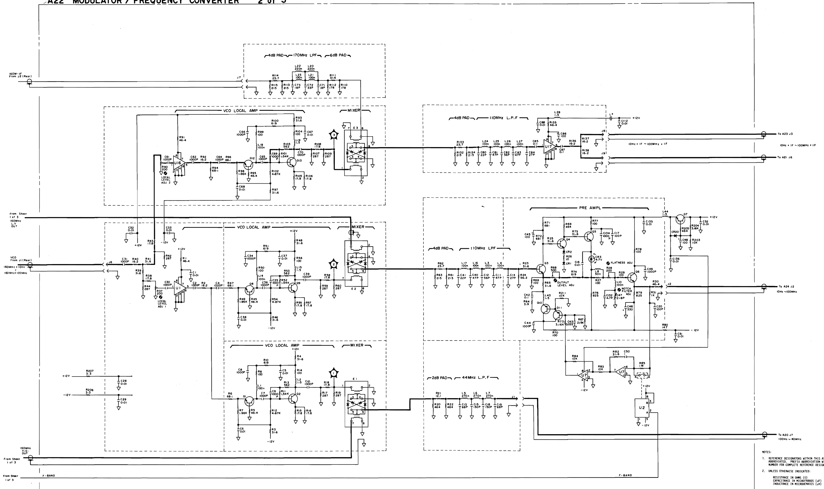
A22 Modulator/Frequency Converter Schematic Diagram (2 of 3)
