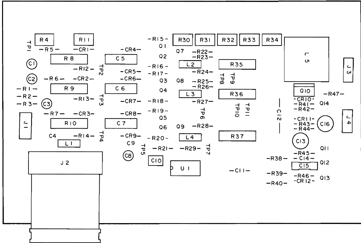
A5 Video Amplifier Component Locations
