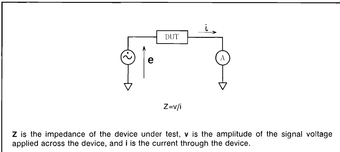
Figure 8-4. Voltage-Current Ratio Measurement Method
