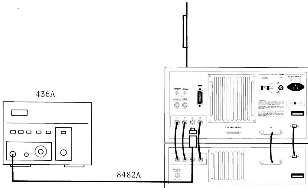
Figure 5-7. 160MHz Signal Output Level Adjustment Setup
