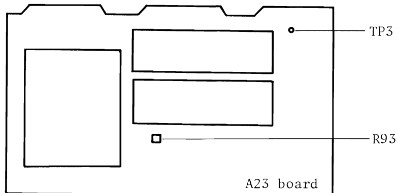
Figure 5-21. A23 Local Oscillator Adjustment Locations
