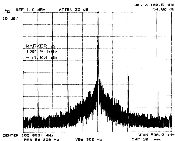
Figure 5-14. Incorrectly Adjusted VCO Output
