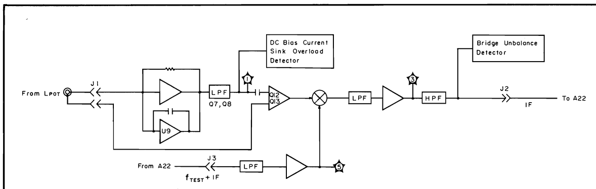
Figure A23-1. A23 Board Block Diagram
