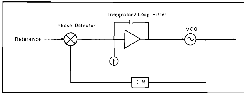
Figure A11-3. Variable Phase PLL with a Current Source
