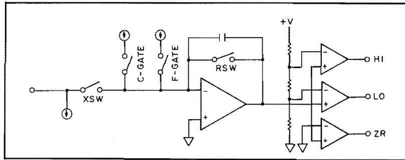
Figure A9-3. Multi-Slope A-D Converter
