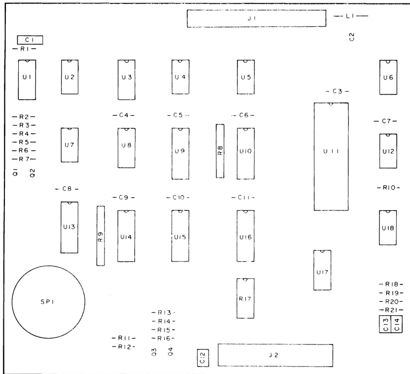
A12 Keyboard Control Component Locations
