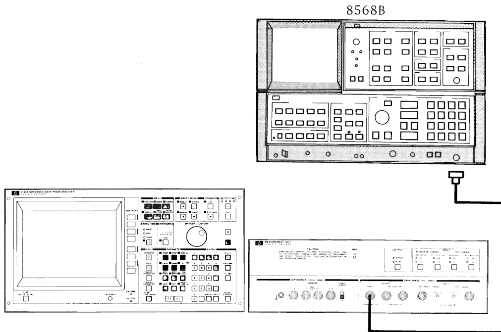
Figure 5-25. 160MHz Notch Filter Adjustment Setup
