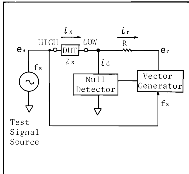
Figure 8-7. Auto-Balanced Bridge Circuit
