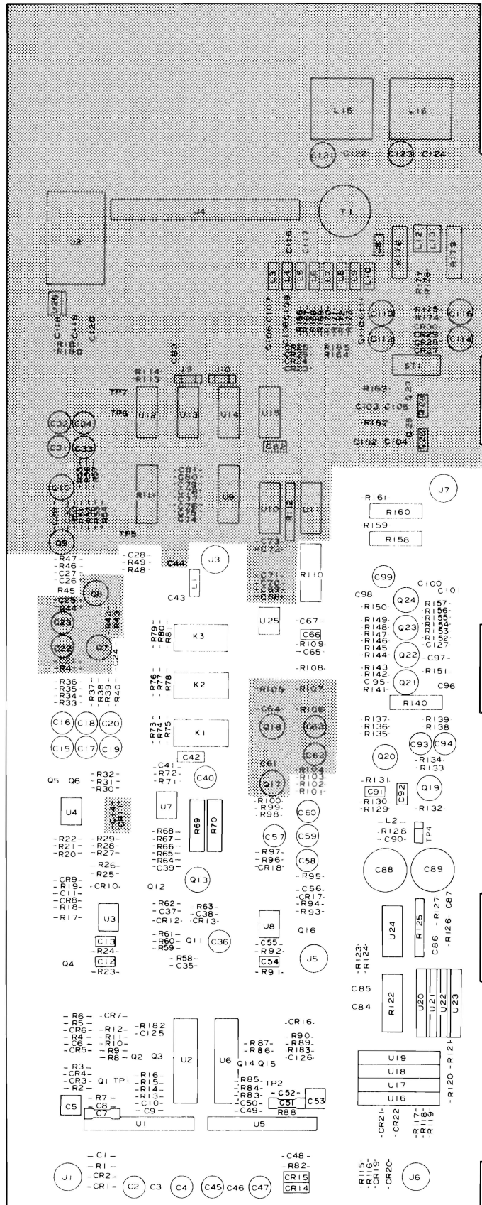
A20 Range Resistor Component Locations (1 of 2)
