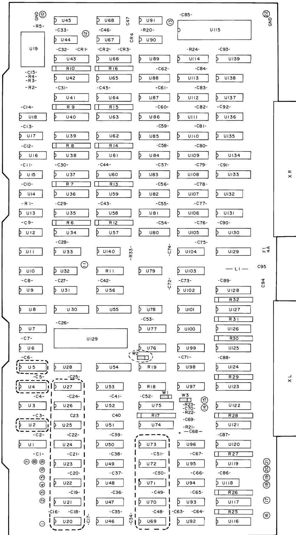
Figure 7-1. A7 Board Component Locations Changes
