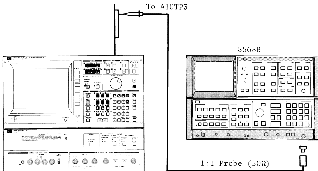
Figure 5-8. 80MHz-IF/2 VCXO Level and Variable Range Adjustment Setup
