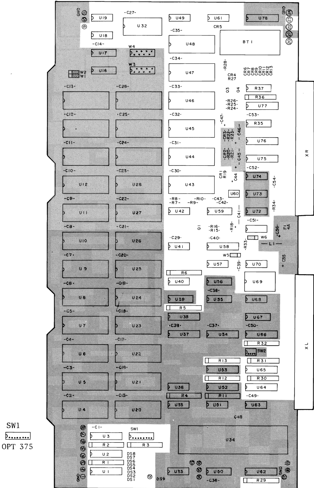
A6 Data Manipulation Processor Component Locations (2 of 2)
