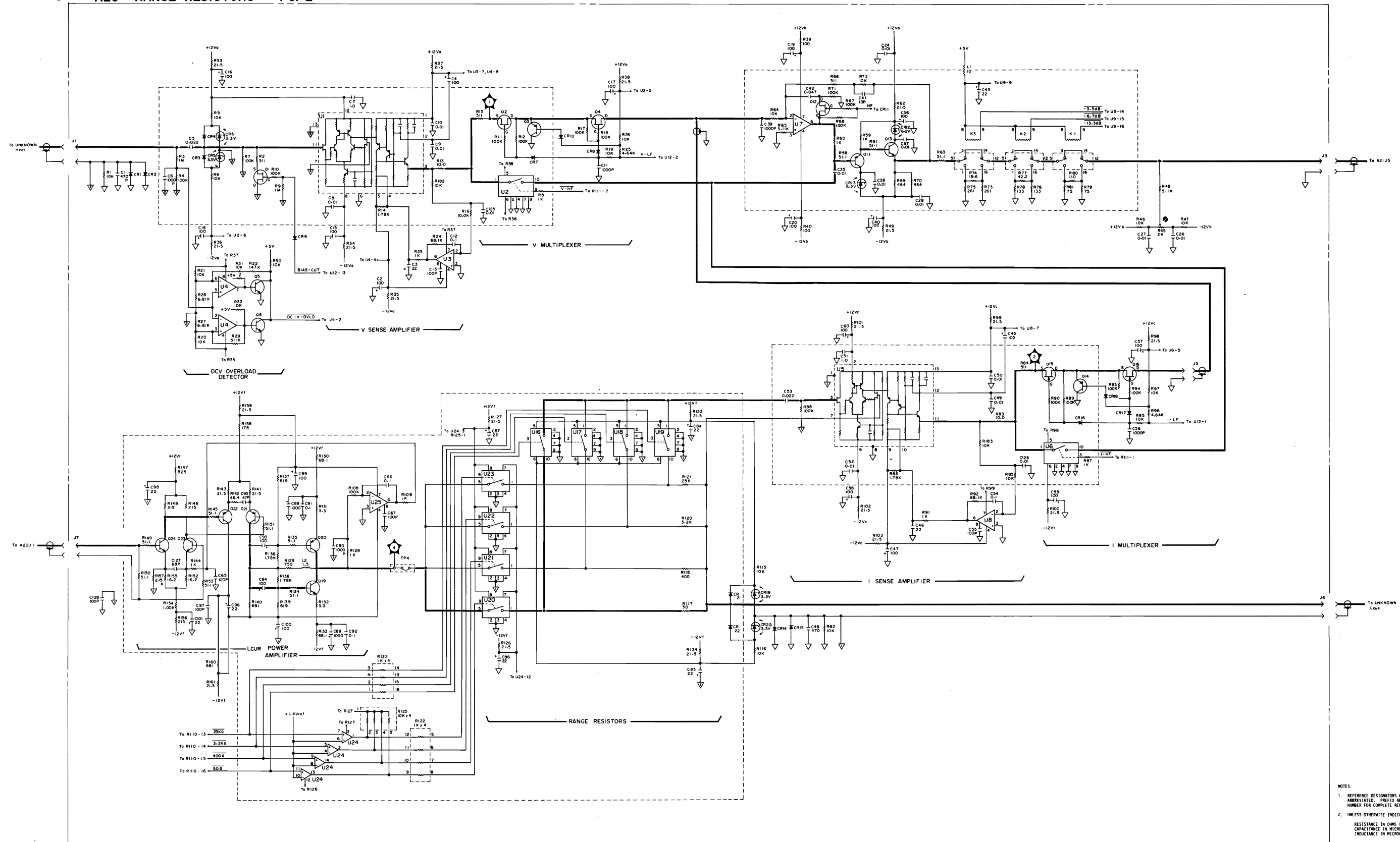
A20 Range Resistor Schematic Diagram (1 of 2)
