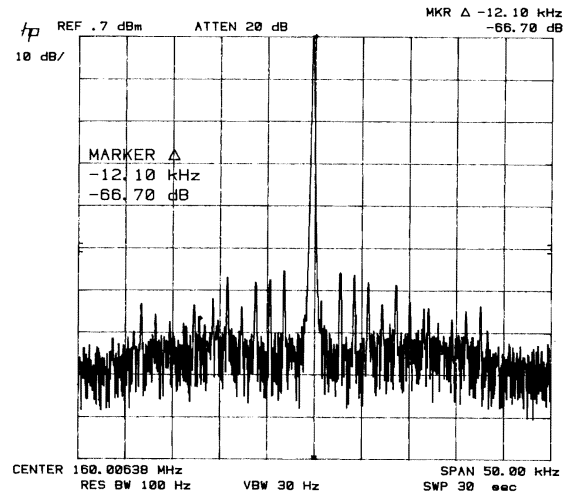
Figure 5-19. Properly Adjusted Spectrum
