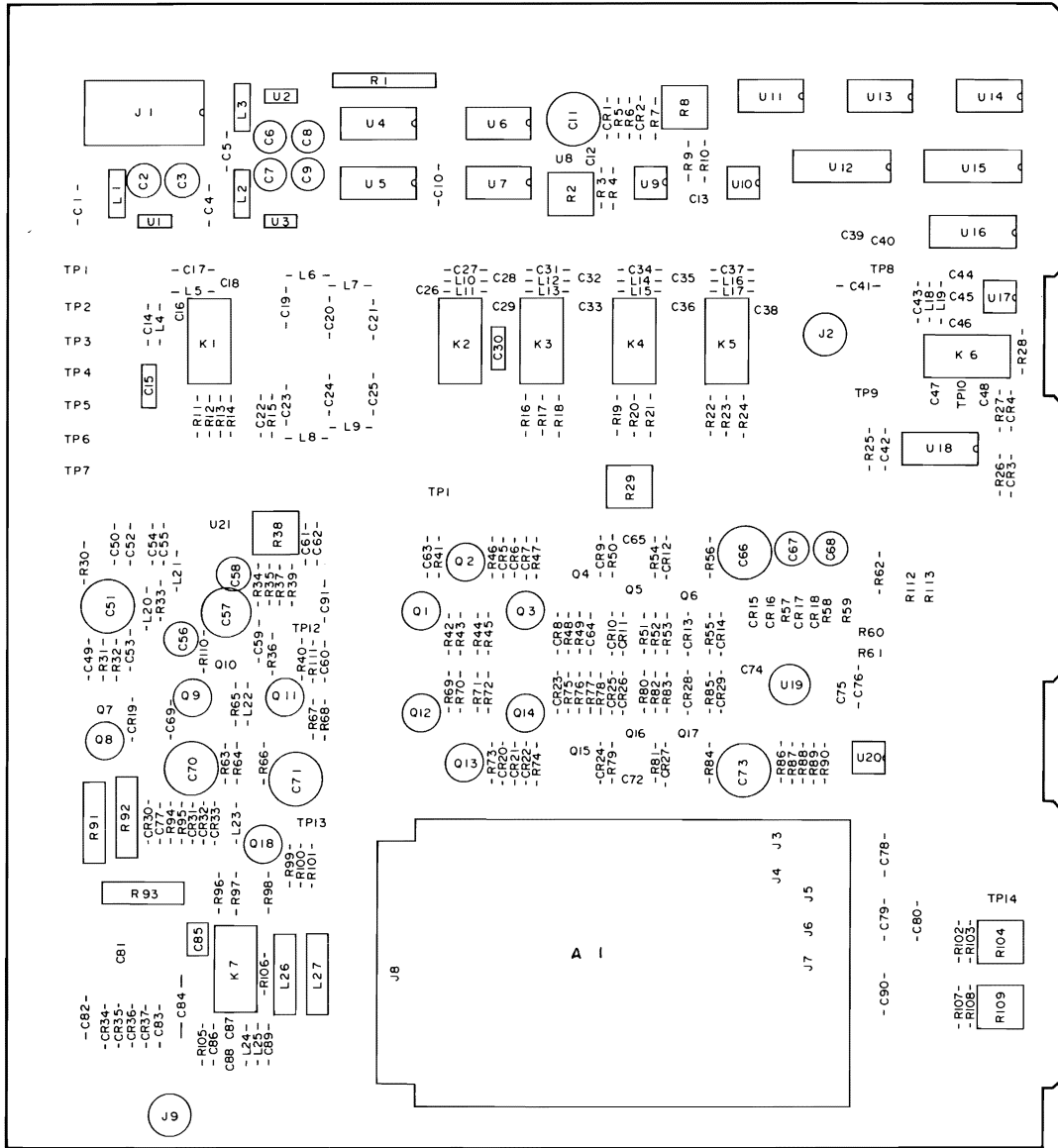
A34 Output Amplifier Component Locations
