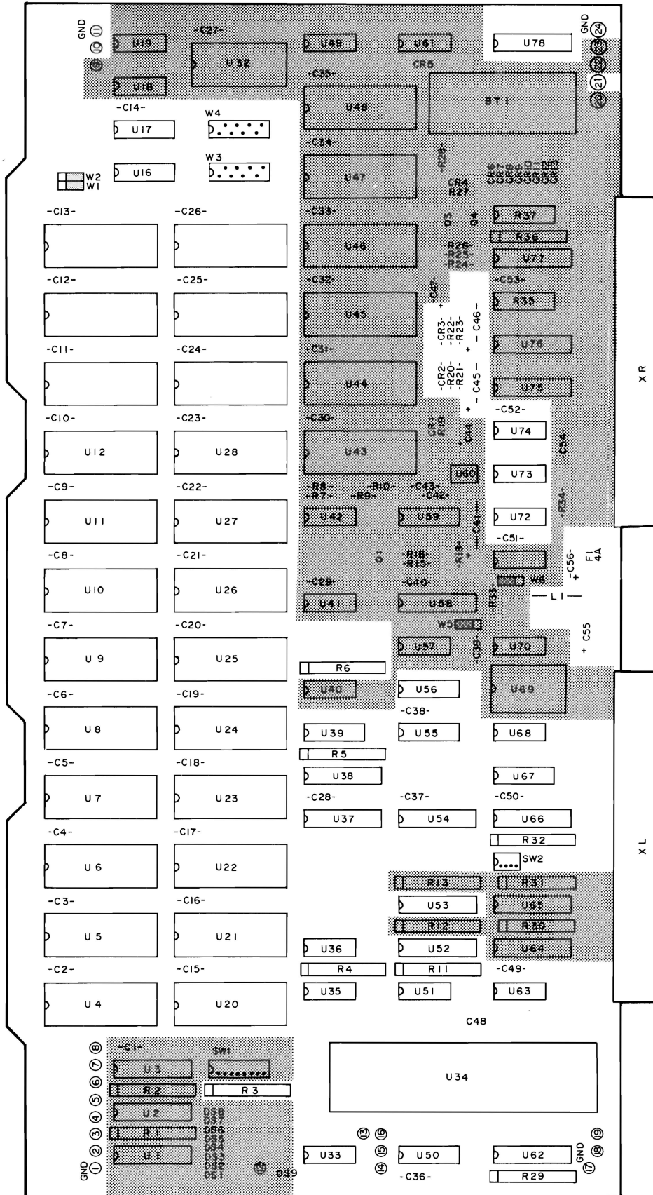
A6 Data Manipulation Processor Component Locations (1 of 2)
