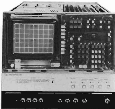
Figure 5-48. Display Position, Size, and Pincushion Adjustment Setup
