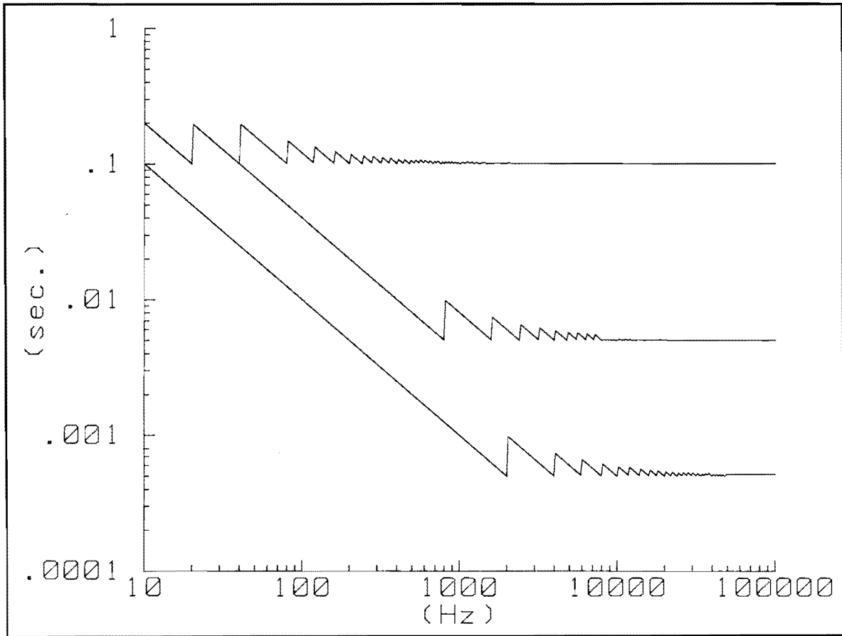
Figure A9-5. INTEG TIME and Measurement Frequency
