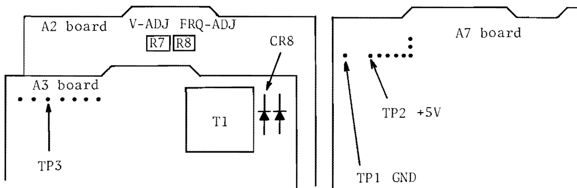
Figure 5-2. Switching Power Supply Adjustment and Test Point Locations
