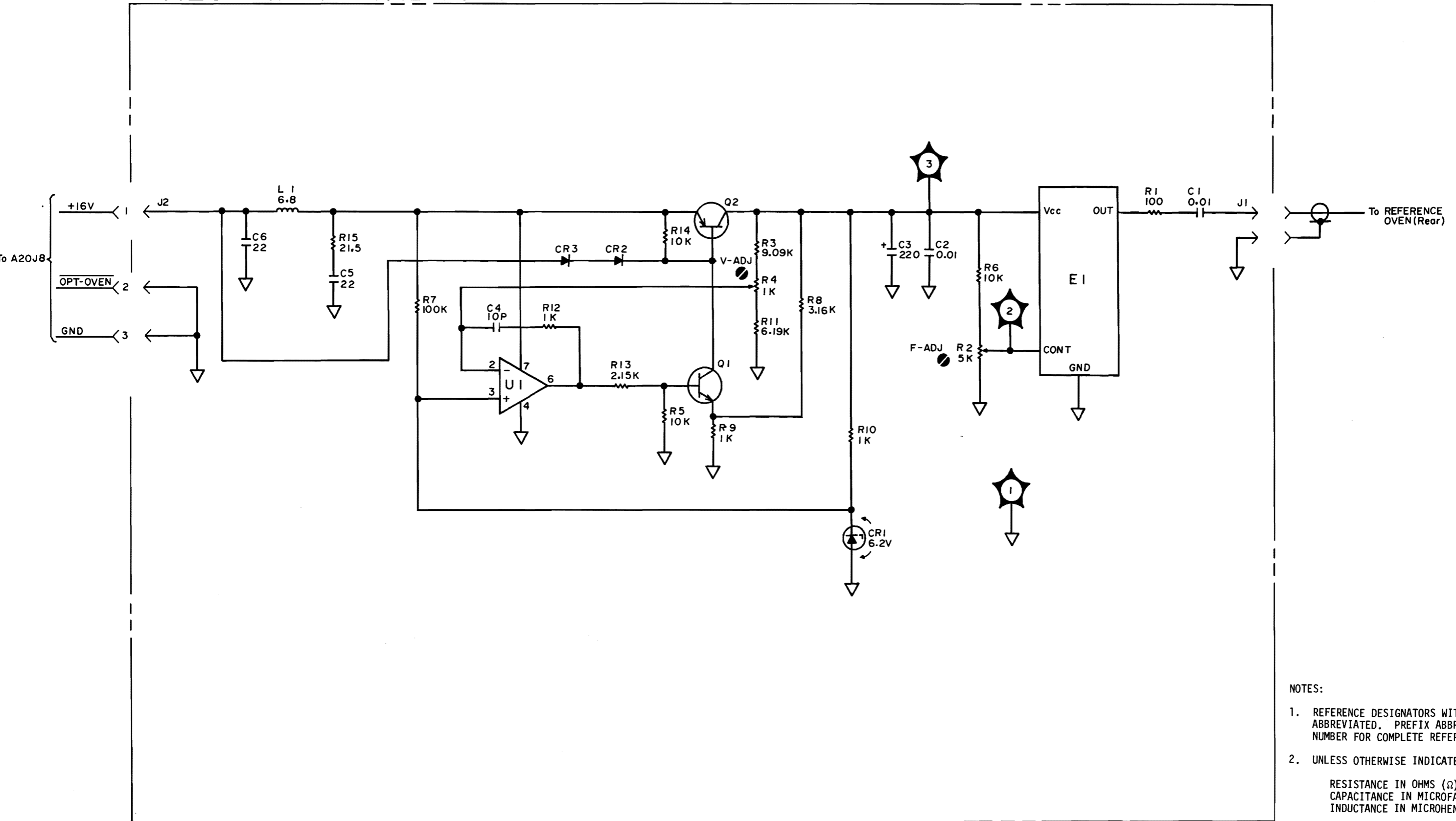
A25 High Stability Oscillator Schematic Diagram
