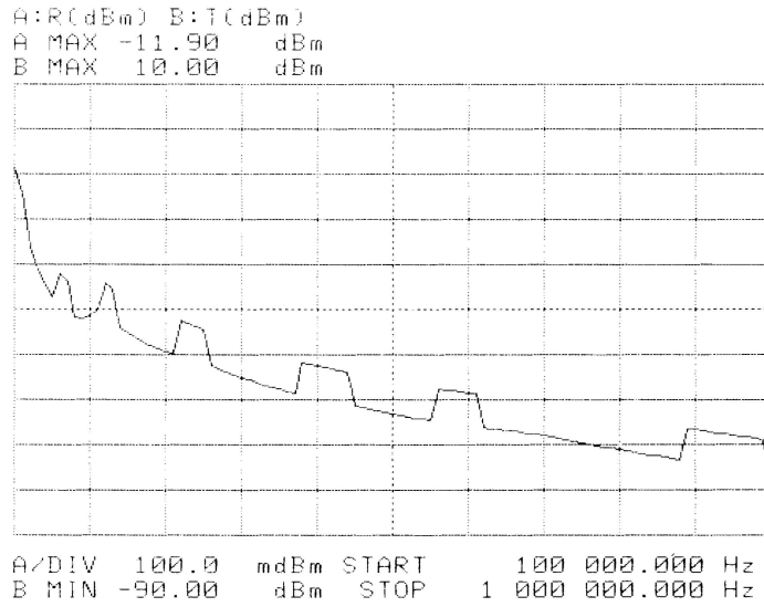
Figure 5-40. Incorrectly Adjusted Trace
