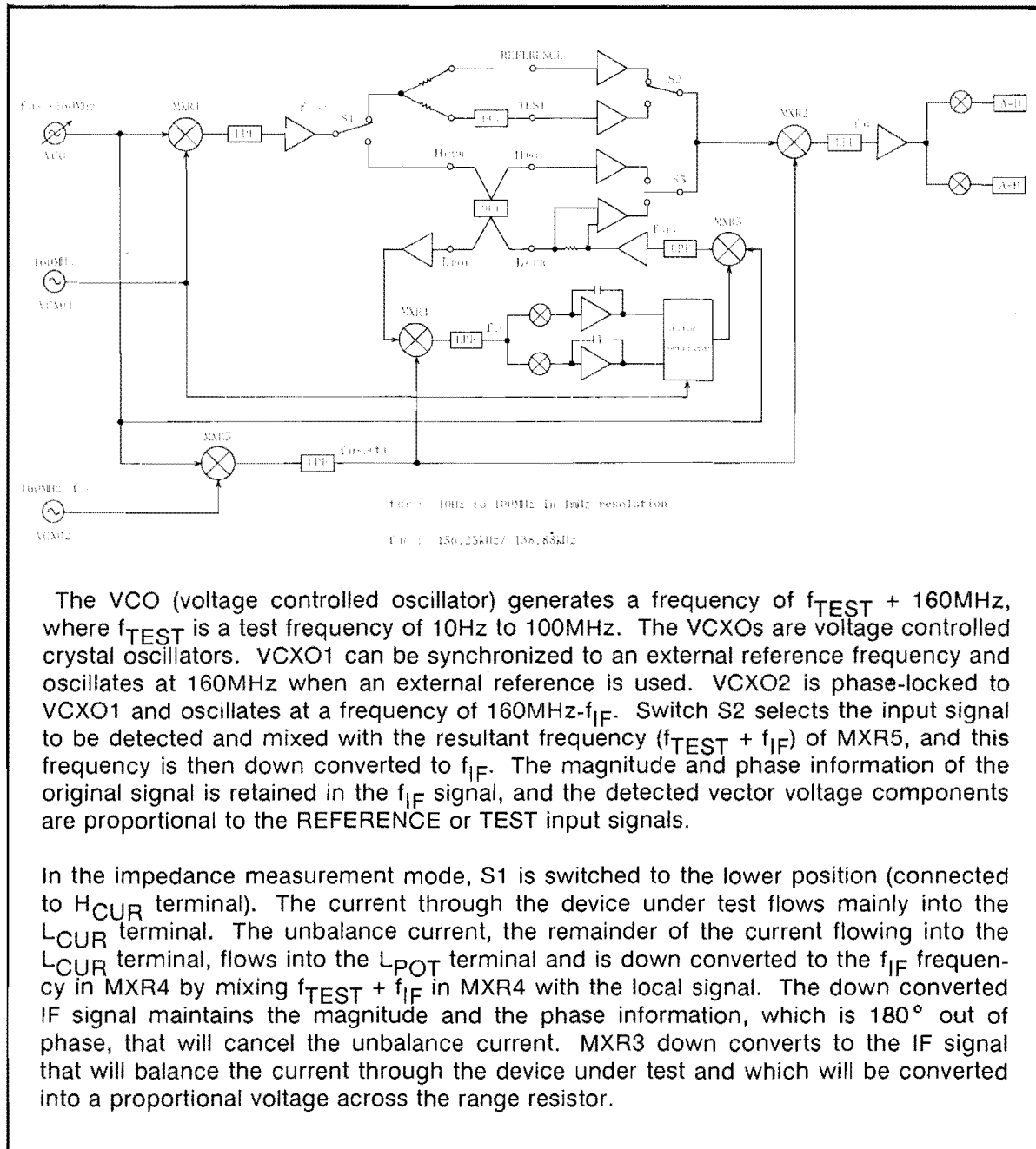
Figure 8-13. Simplified Block Diagram Discussion
