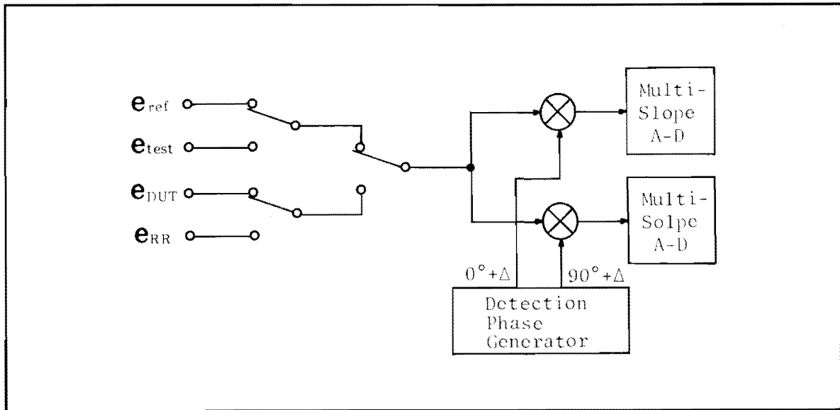
Figure 8-15. 4194A's VVD Section
