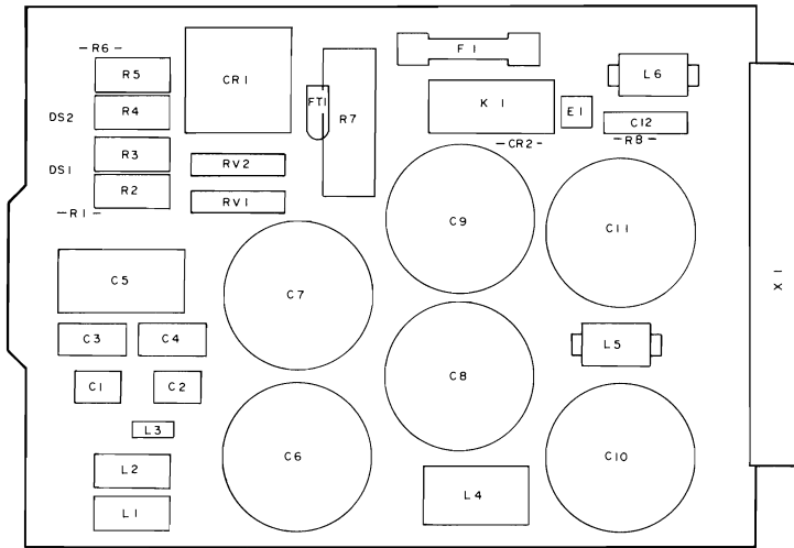
A1 Primary Rectifier Component Locations
