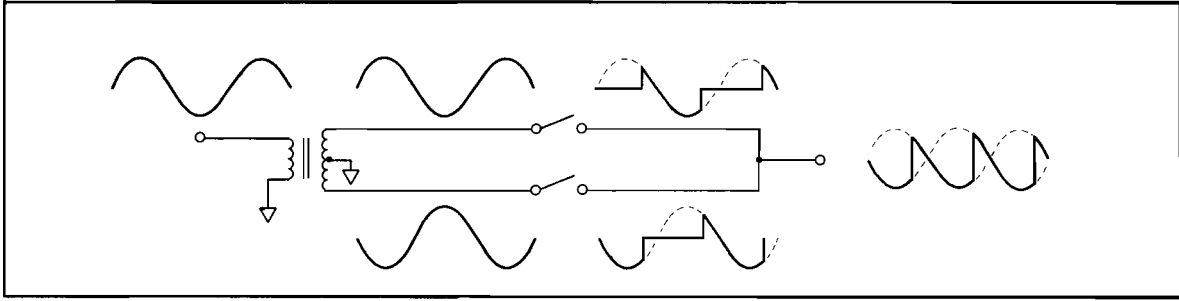
Figure A9-2. Double Wave Phase Detection Example
