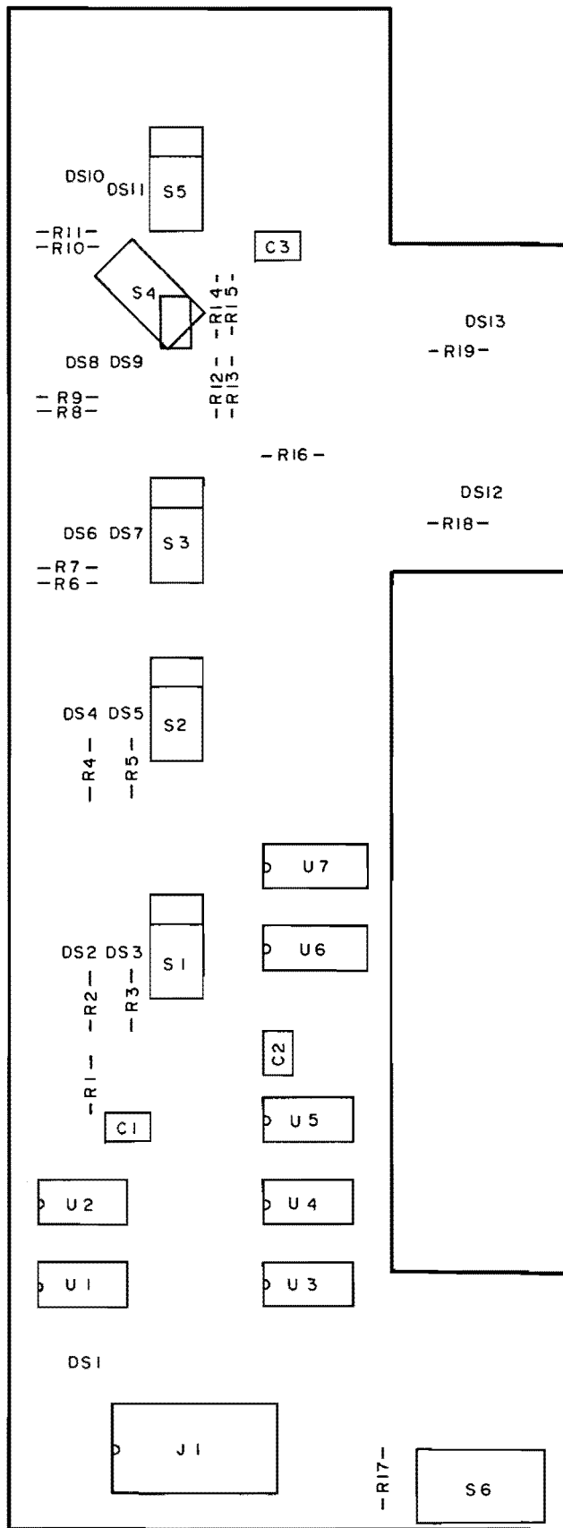
A26 Measurement Unit Keyboard Component Locations 8-168
