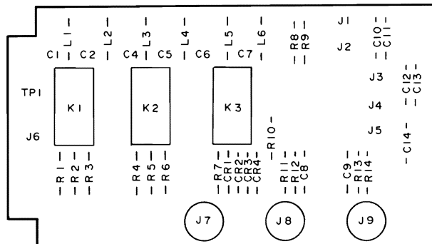
A34A1 Attenuator/Power Splitter Component Locations
