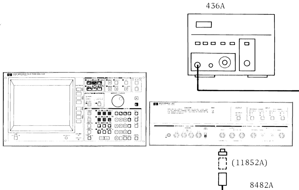
Figure 5-27. Test Signal Level and Flatness Adjustment Setup
