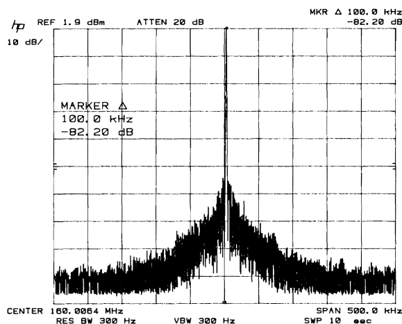
Figure 5-15. Properly Adjusted VCO Output
