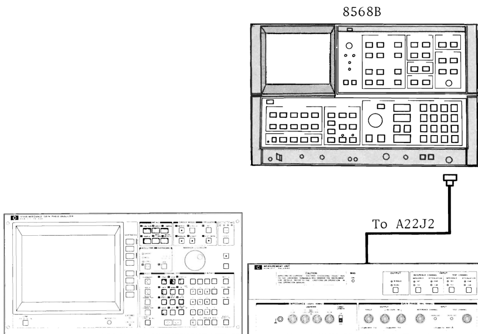
Figure 5-26. Mixer Local Level Adjustment Setup
