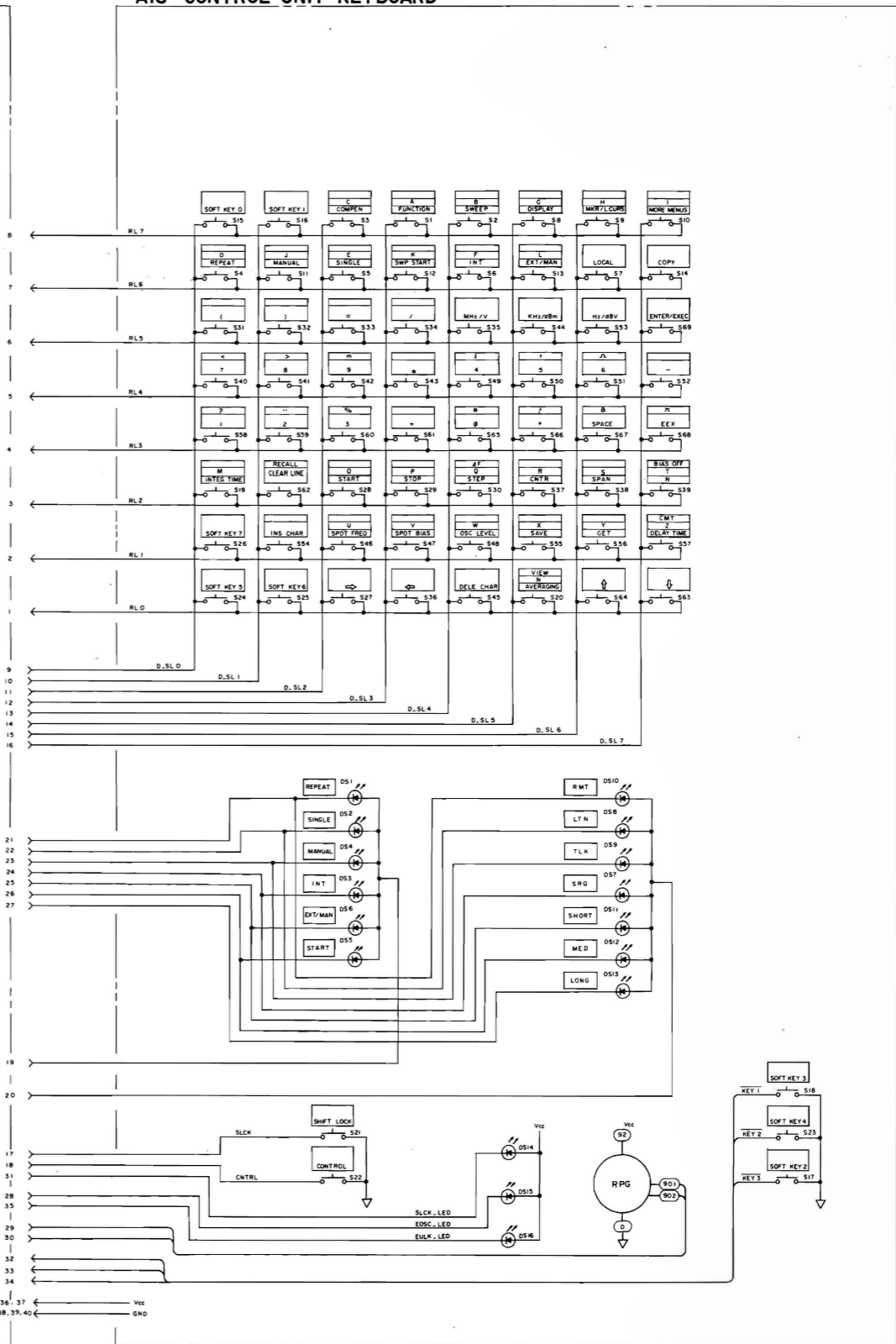
A12/A13 Control Unit Keyboard Schematic Diagrams
