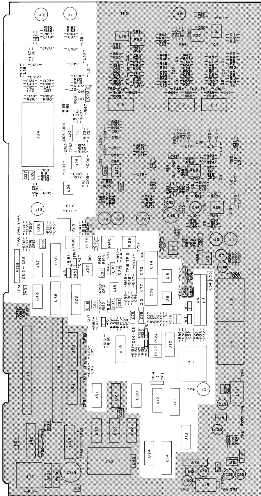
A22 Modulator/Frequency Converter Component Locations (1 of 3)
