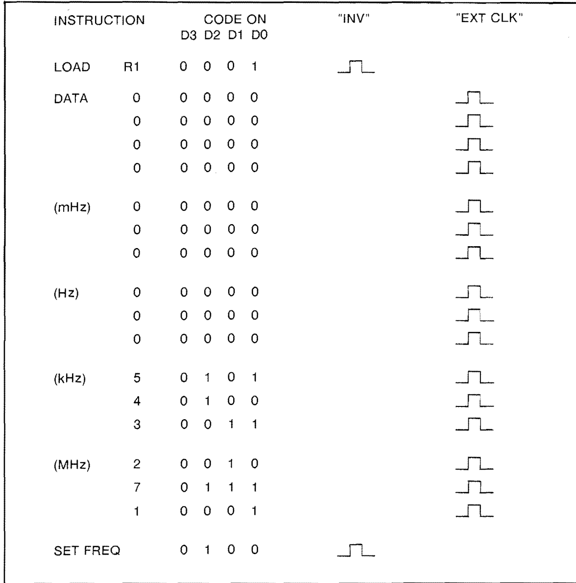
Figure A8-2. Fraction N Loop Setup Example
