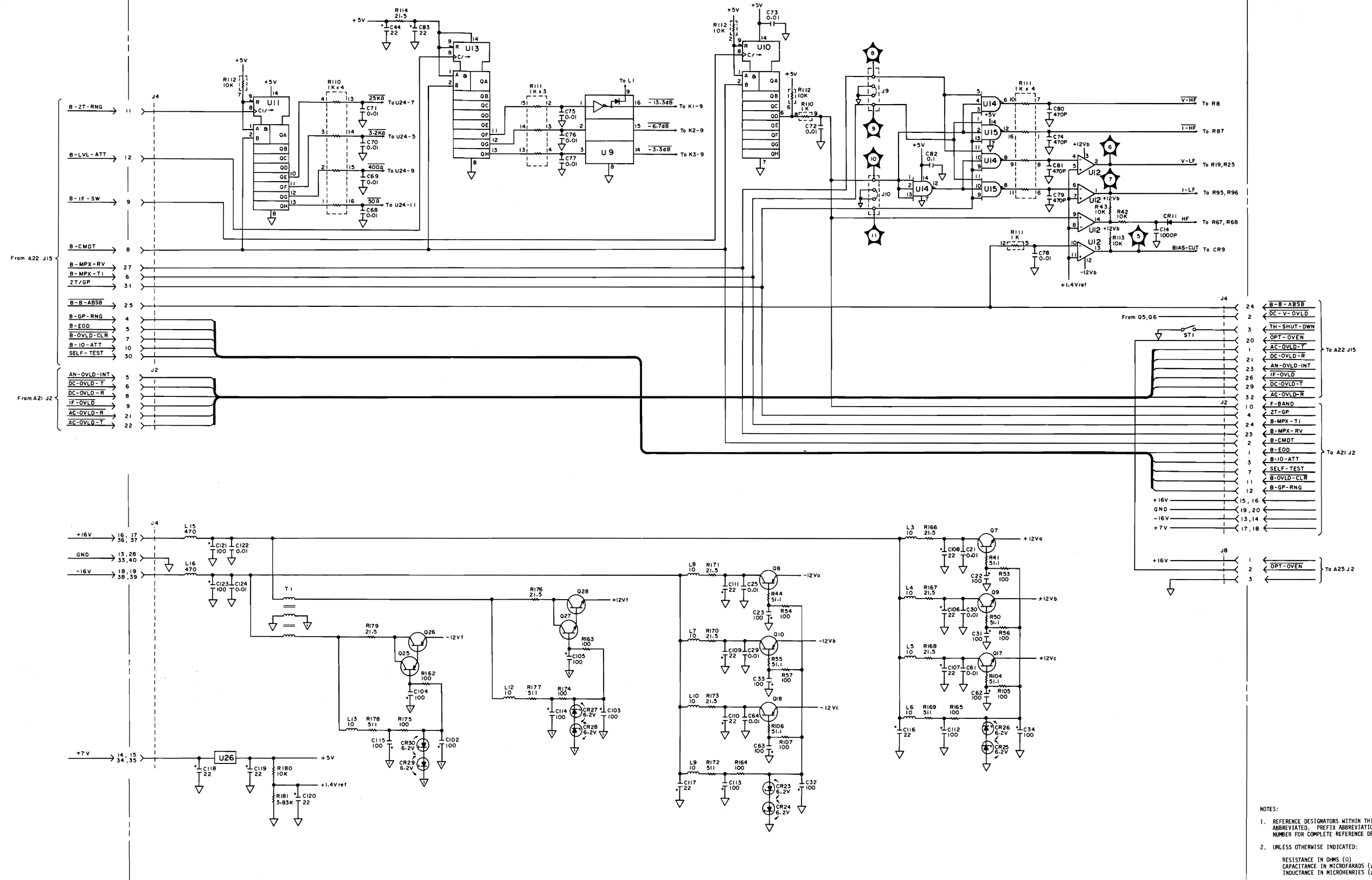
A20 Range Resistor Schematic Diagram (2 of 2)
