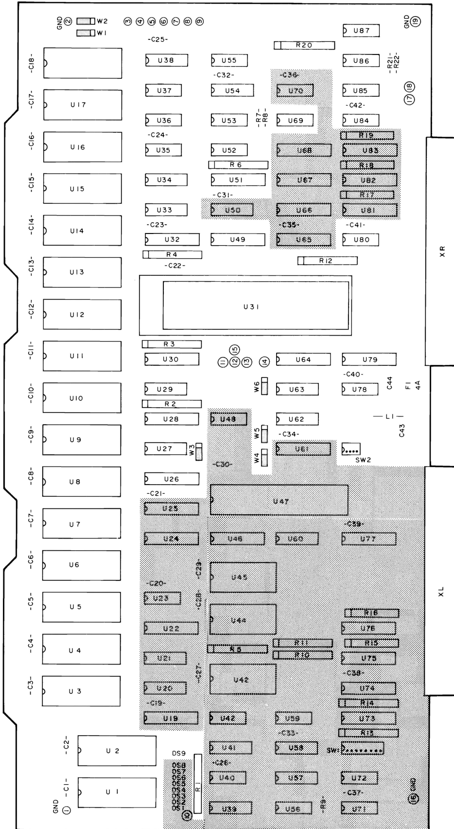
A8 Measurement Control Processor Component Locations (1 of 3)
