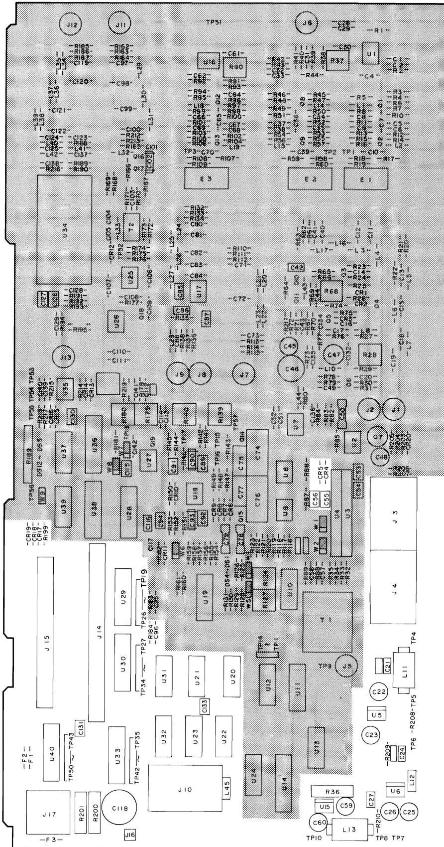
A22 Modulator/Frequency Converter Component Locations (3 of 3)
