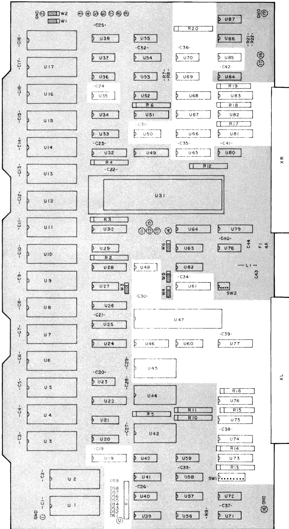
A8 Measurement Control Processor Component Locations (2 of 3)
