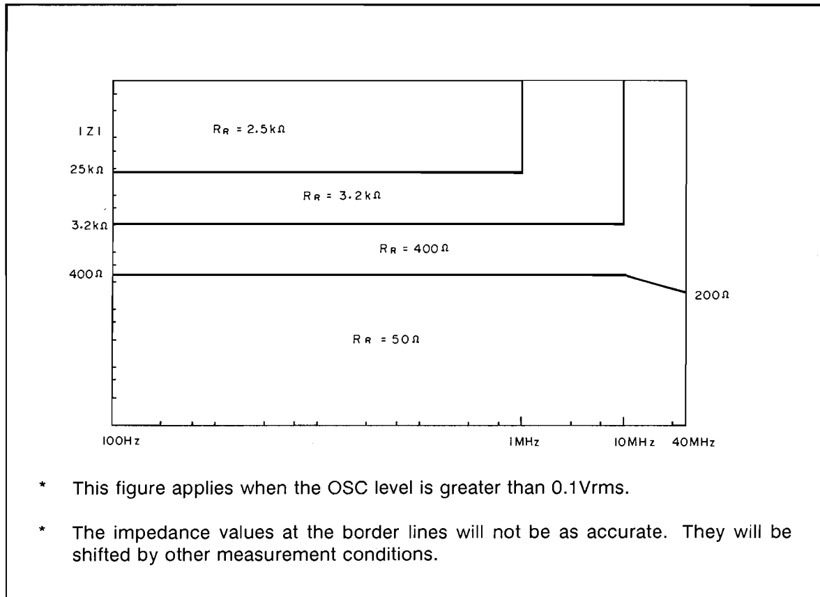
Figure A20-2. Range Resistor Selection
