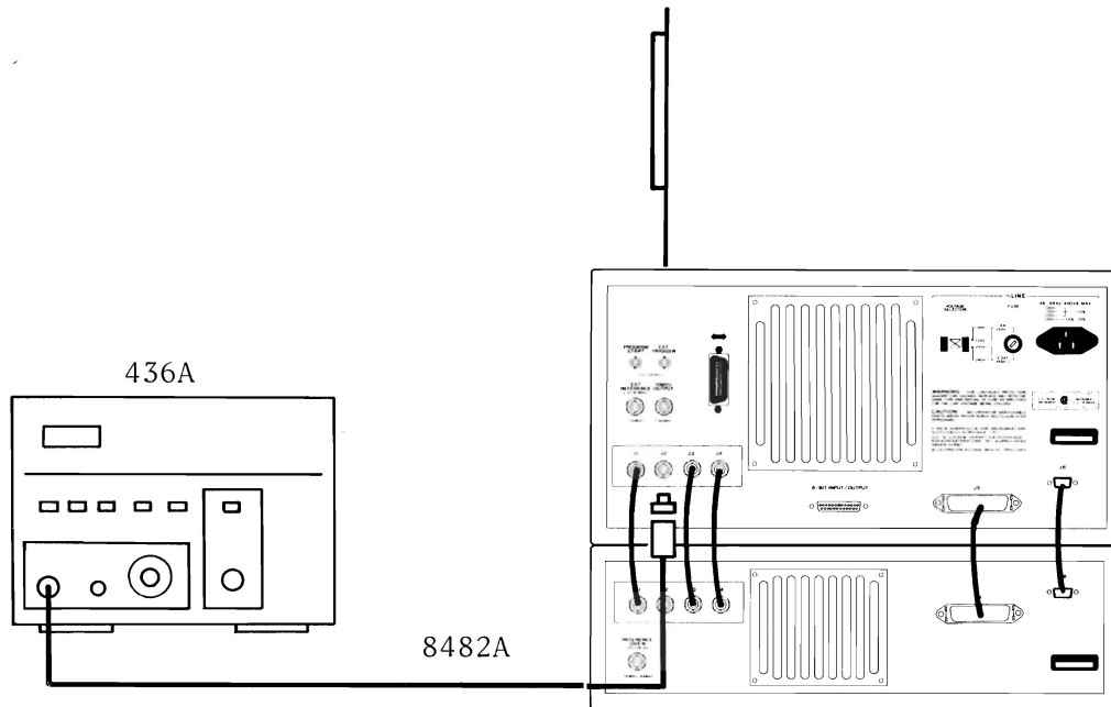
Figure 5-9. 160MHz-IF Signal Level Adjustment Setup
