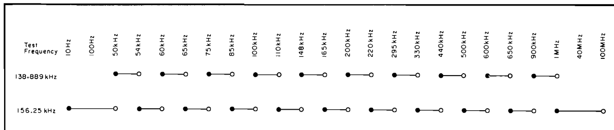
Figure A10-2. Test Frequency and IF Relationship
