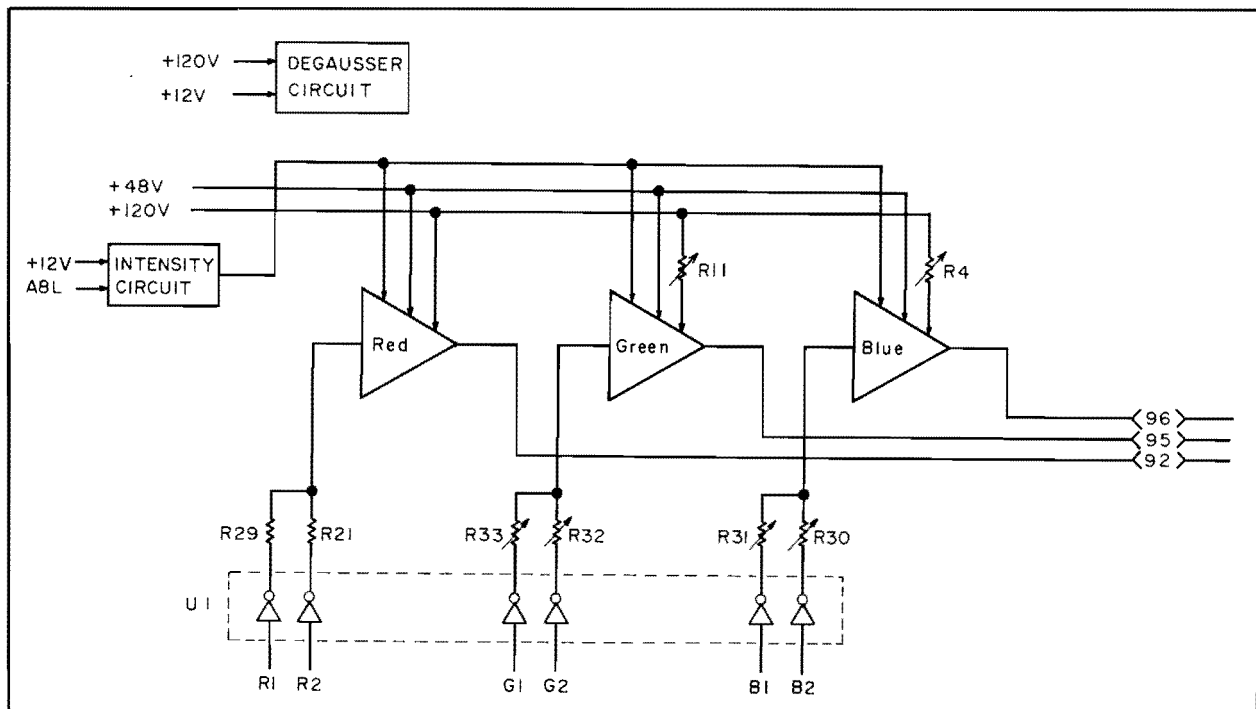
Figure A5-1. A5 board Block Diagram
