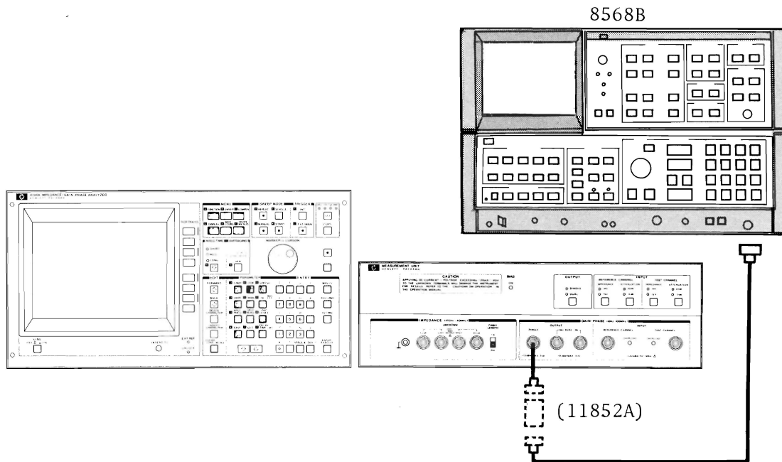
Figure 5-28. Power Amplifier Distortion Adjustment Setup
