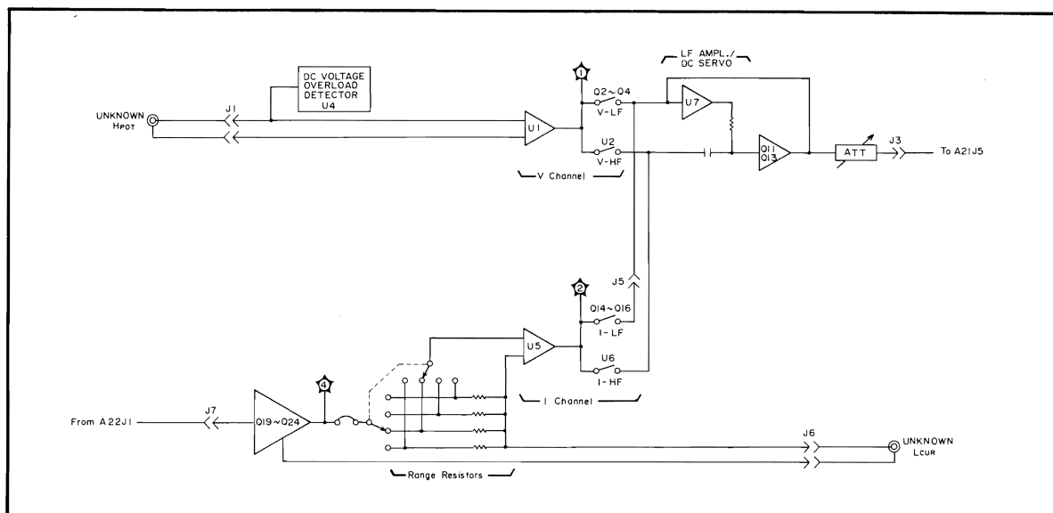
Figure A20-1. A20 Board Block Diagram
