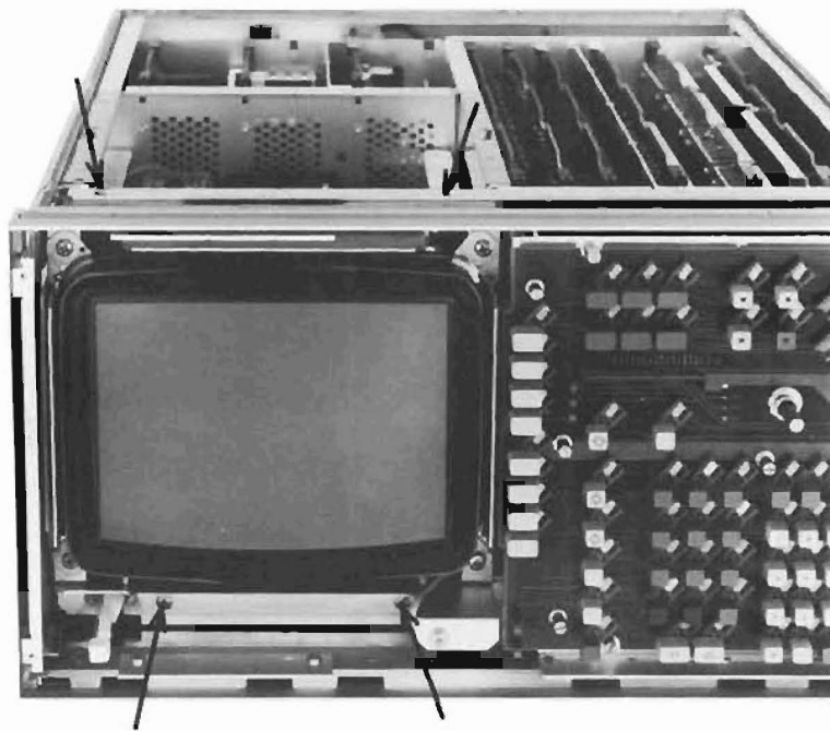
Figure 8-3. Disassembly (sheet 1 of 3)
