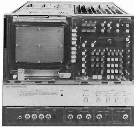
Figure 5-51. Focus and Convergence Adjustment
