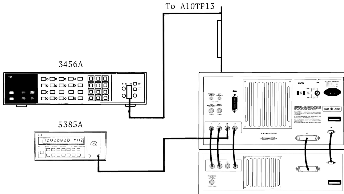
Figure 5-6. 80MHz VCXO Frequency Adjustment Setup
