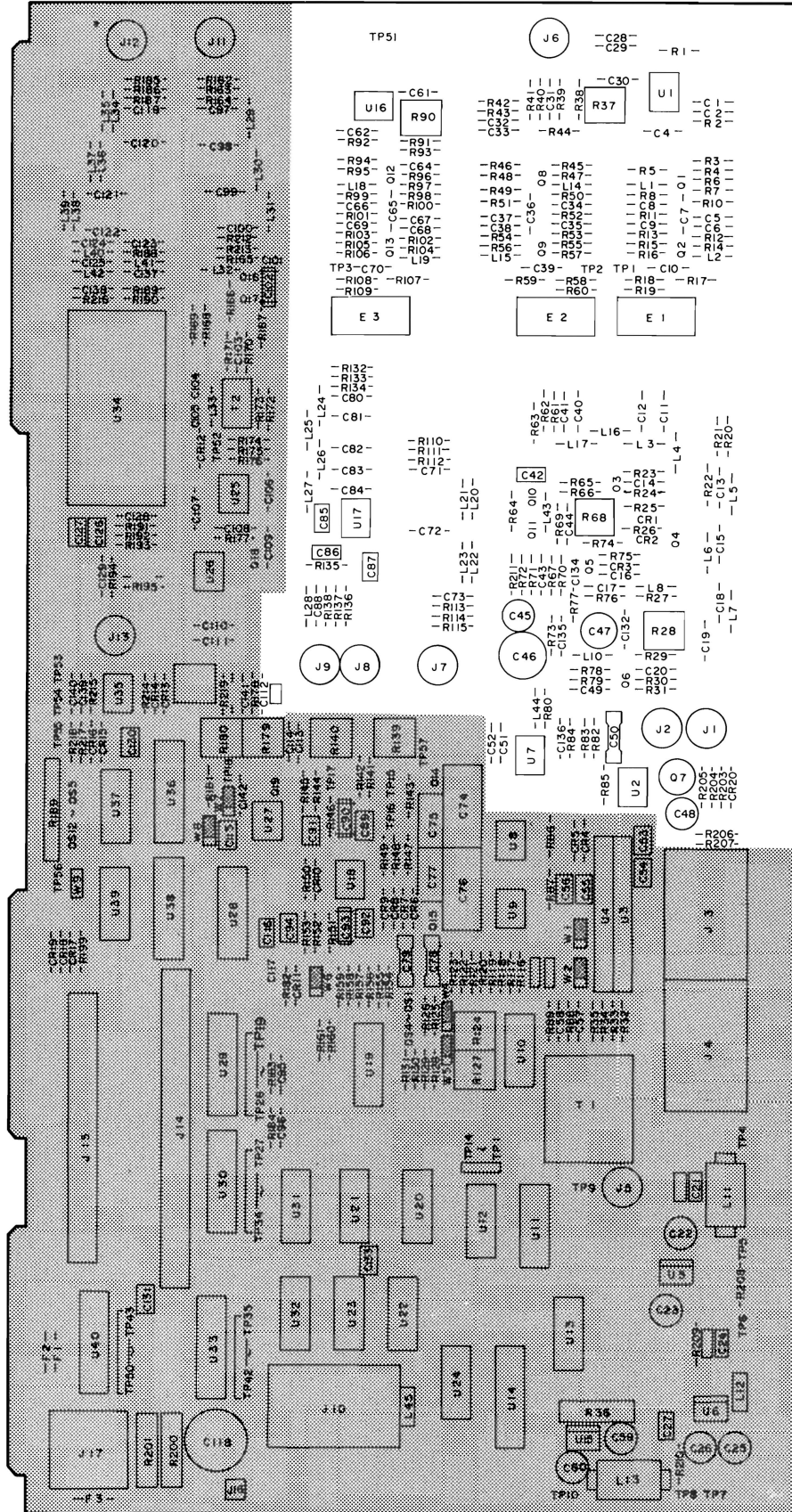
A22 Modulator/Frequency Converter Component Locations (2 of 3)
