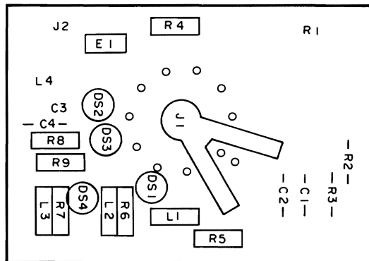
A17 CRT Socket Component Locations
