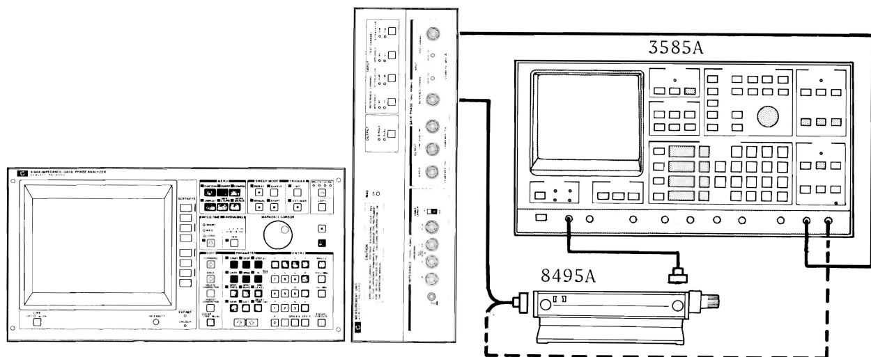
Figure 5-34. IF Band Pass Filter Coarse Adjustment Setup
