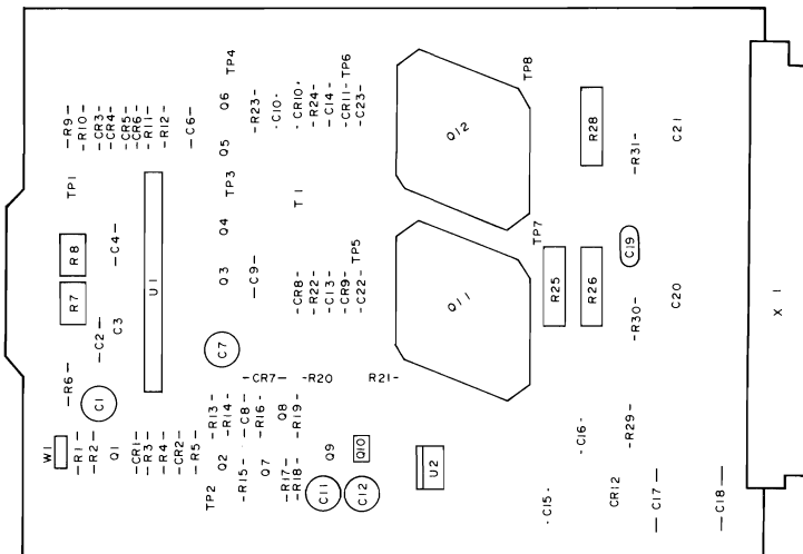
A2 Power Supply Control Component Locations
