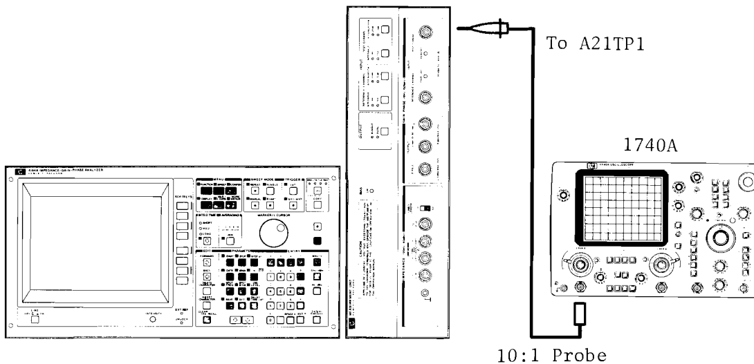
Figure 5-37. Mixer Local Feedthrough Adjustment Setup
