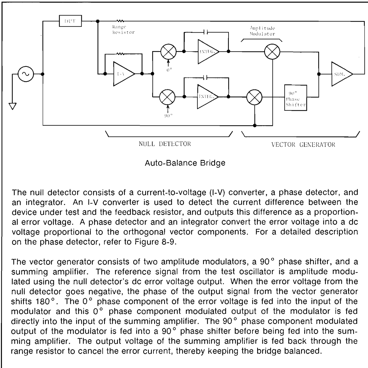
Figure 8-8. Auto-Balance Bridge Operating Principle
