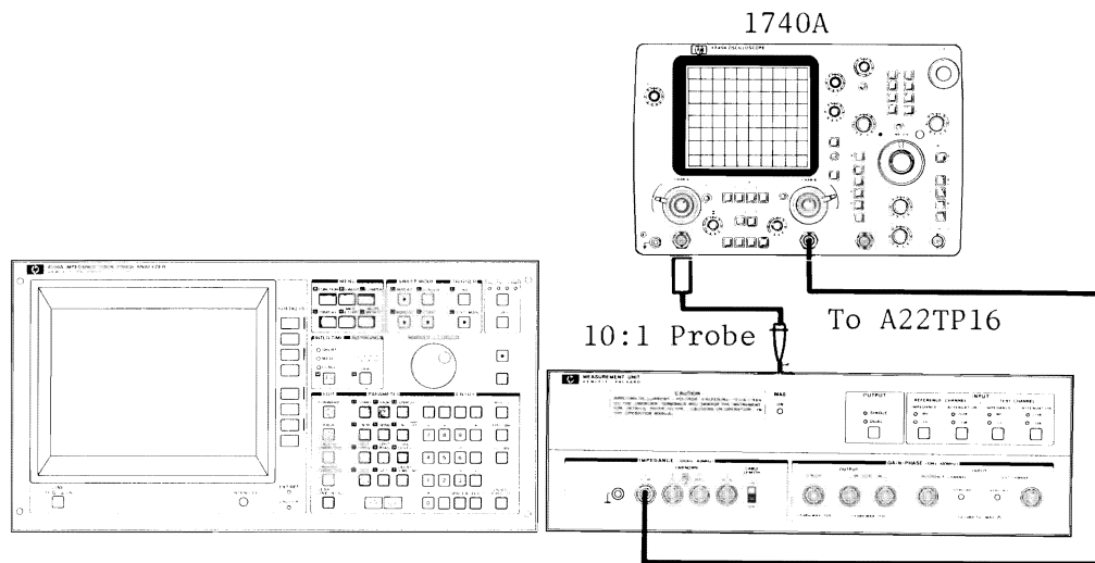
Figure 5-22. L CUR Output Adjustments Setup
