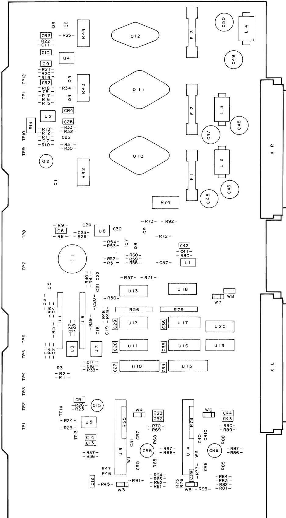
A9 Phase Detector/A-D Converter Component Locations 8-100
