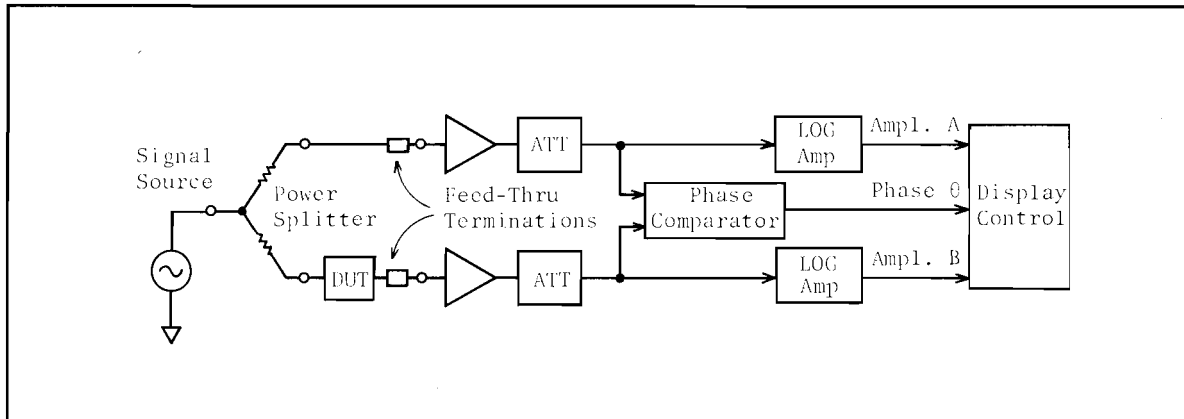
Figure 8-11. Typical Network Analyzer Construction
