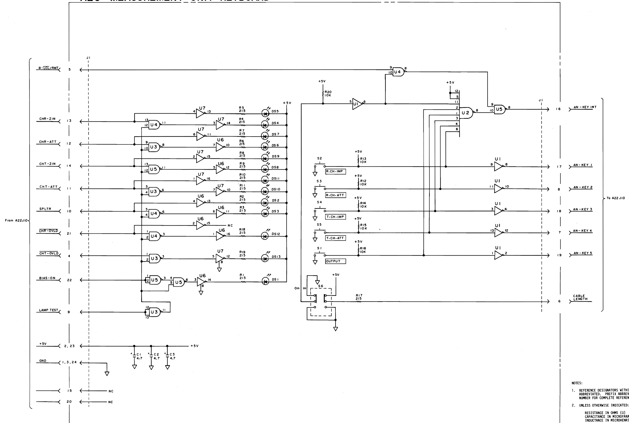
A26 Measurement Unit Keyboard Schematic Diagram
