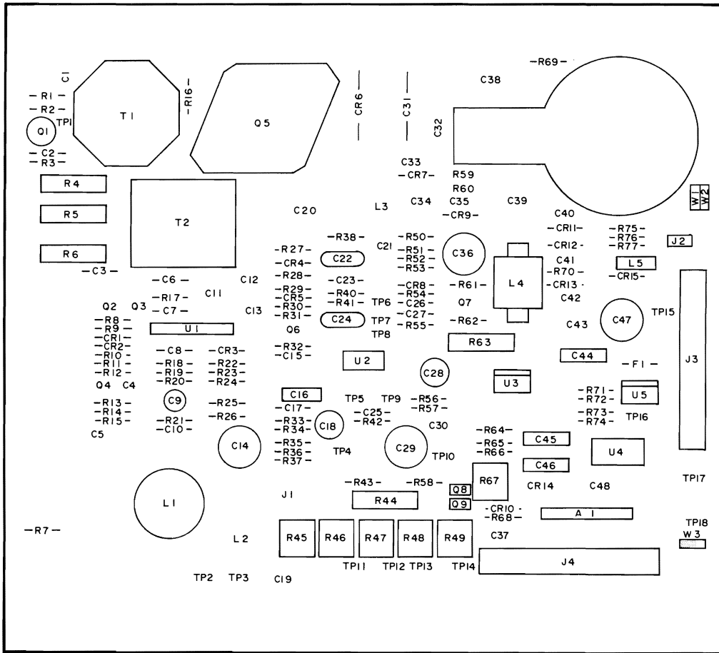
A4 CRT Deflection Component Locations
