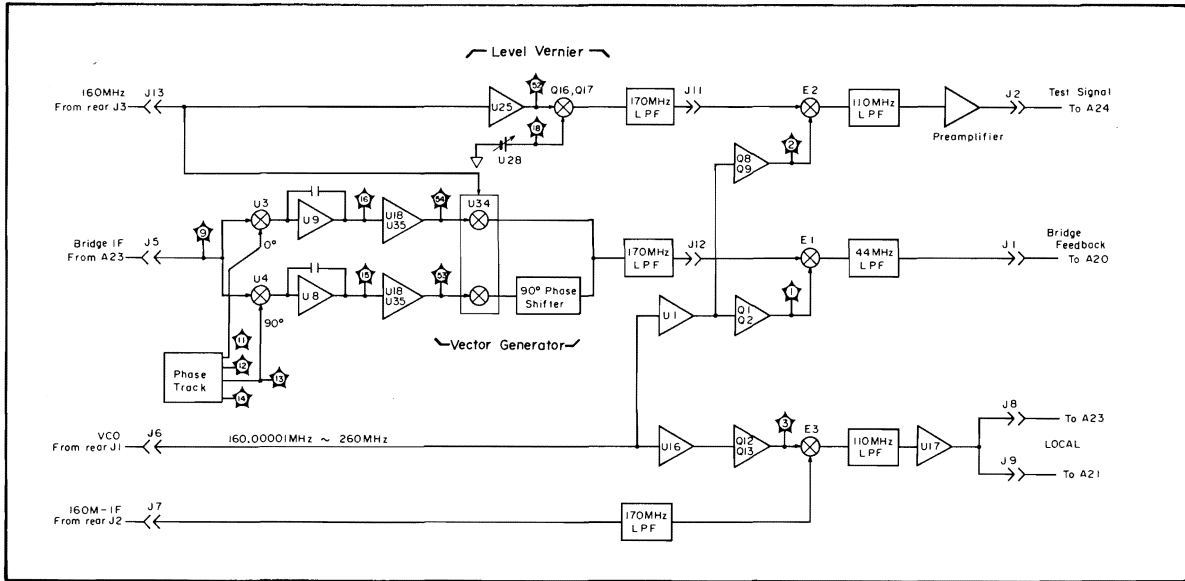
Figure A22-1. A22 Board Block Diagram
