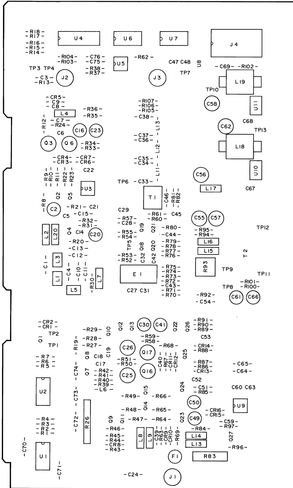
A23 Null Detector Component Locations
