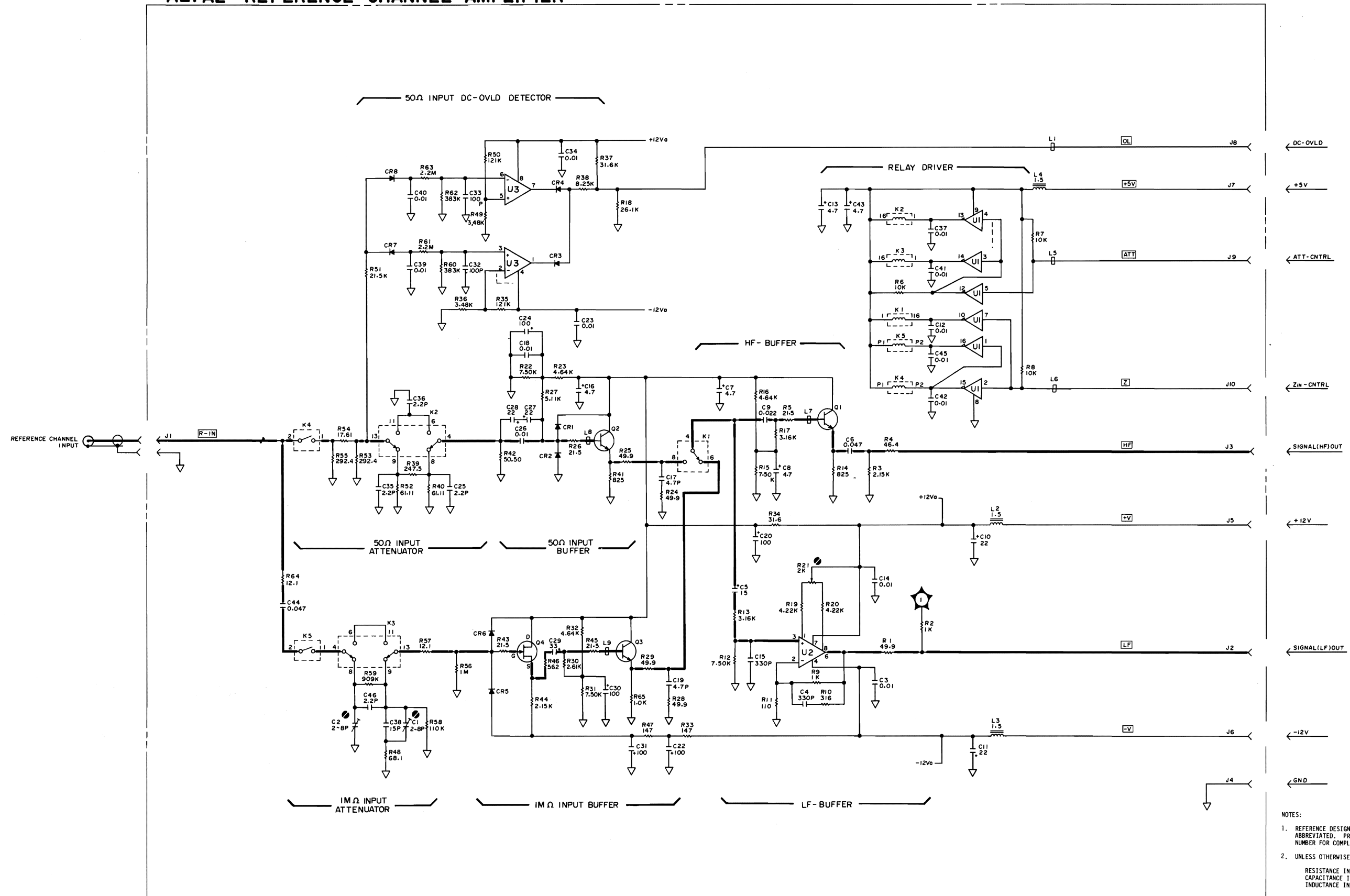
A21A2 Reference Channel Amplifier Schematic Diagram
