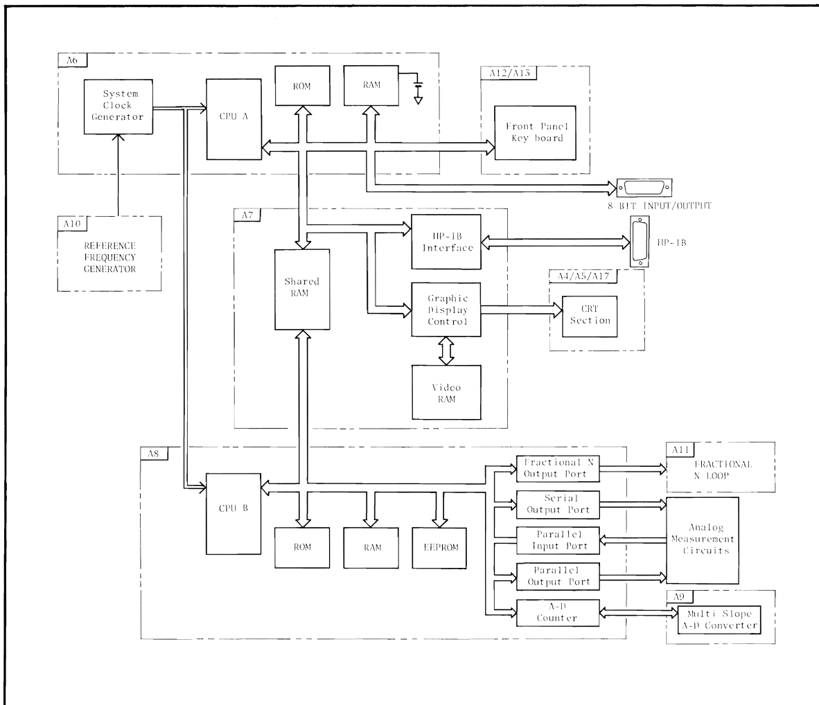
Figure 8-16. Digital Control Section Block Diagram
