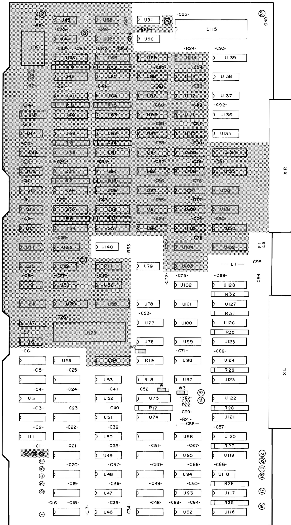
A7 GDC/RAM Component Locations (1 of 2)
