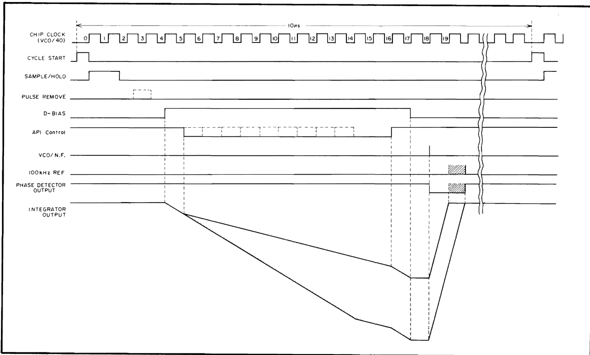
Figure A11-4. Fractional N Loop Timing Diagram
