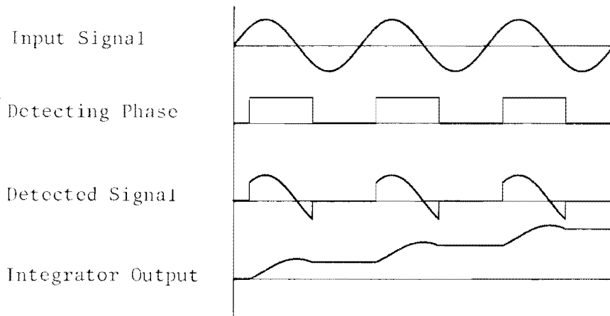
Figure B. VVD Waveforms
