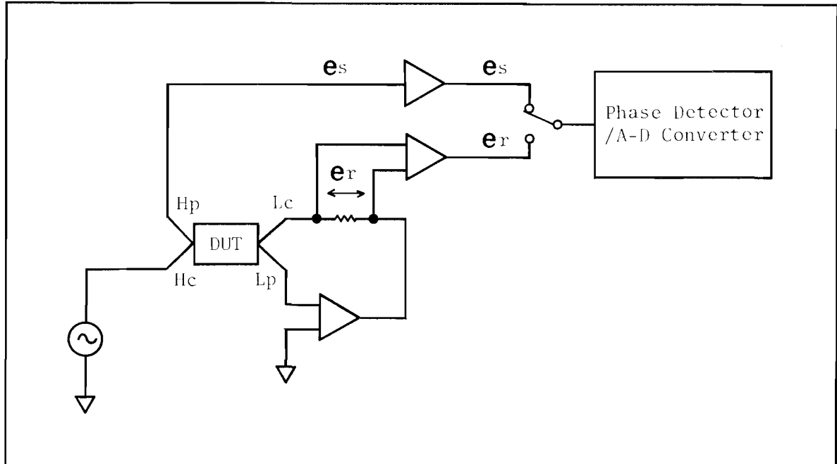
Figure 8-10. Impedance Measurement Circuit
