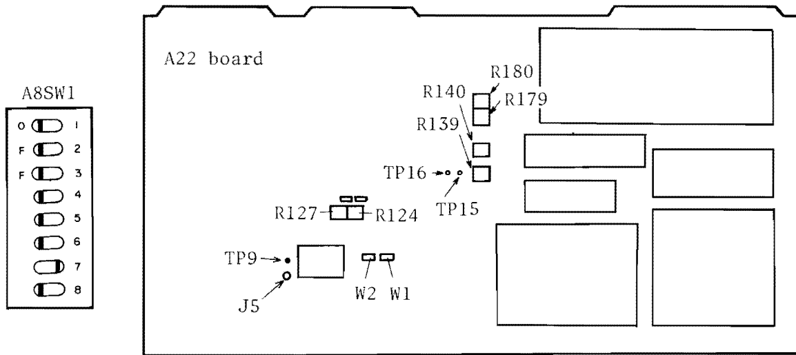
Figure 5-23. Lcur Output Adjustment Locations
