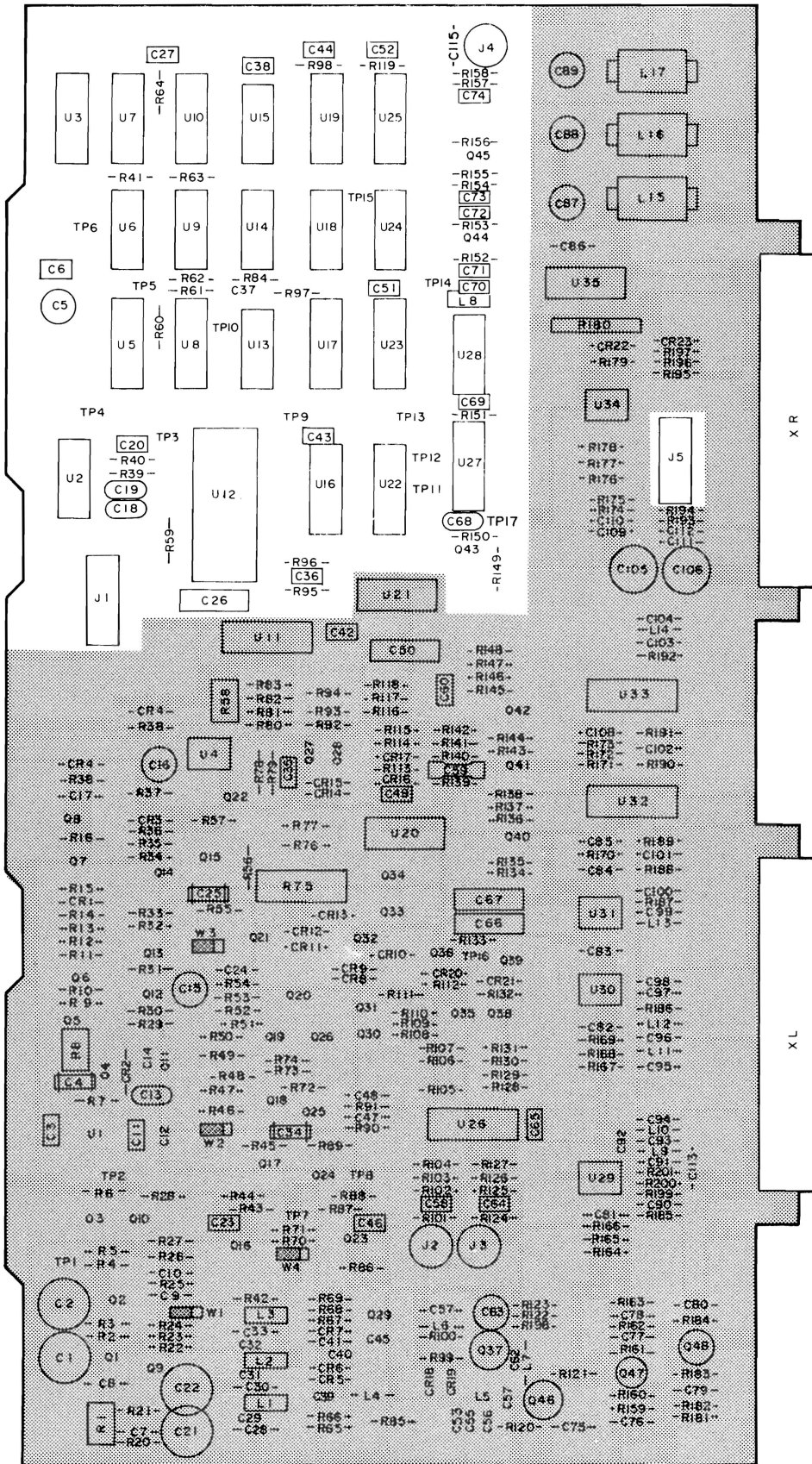
A11 Fractional N Loop Component Locations (2 of 2) 8-117
