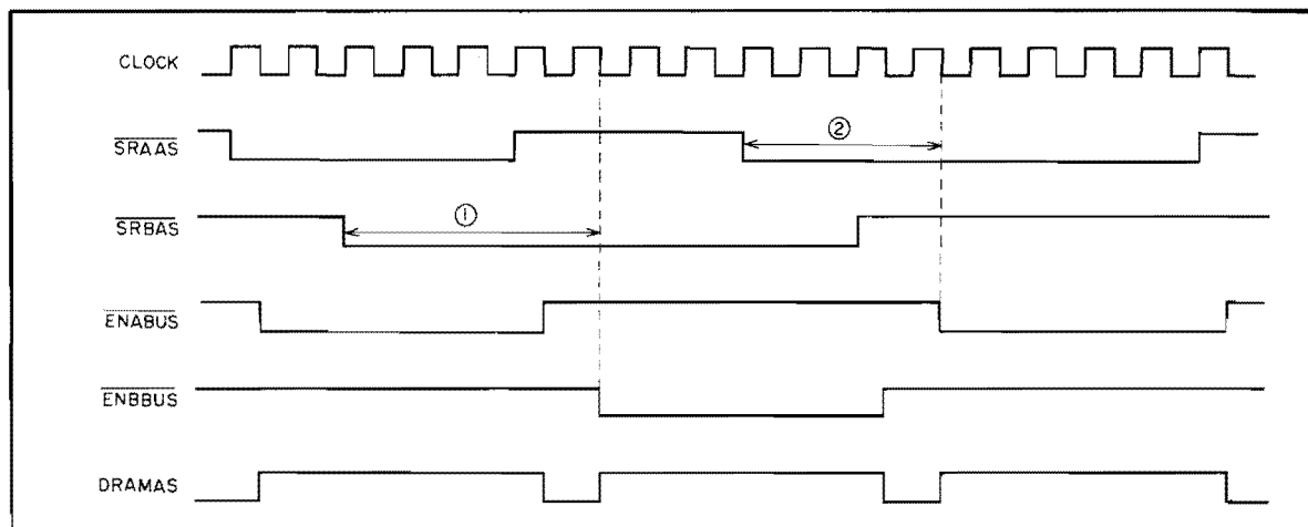
Figure A7-2. Shared RAM Timing Chart
