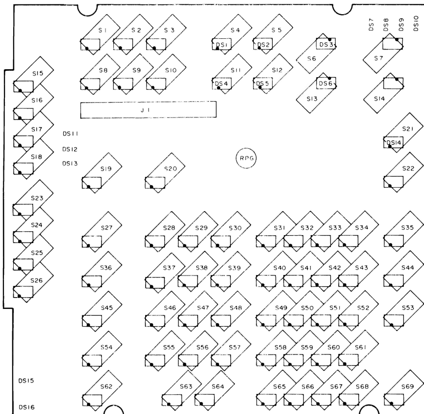
A13 Control Unit Keyboard Component Locations
