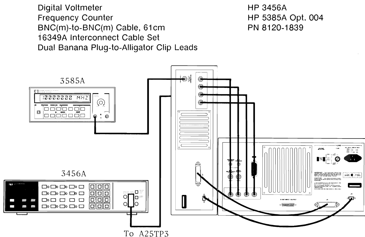
Figure 5-3. High Stability Oscillator Adjustment Setup
