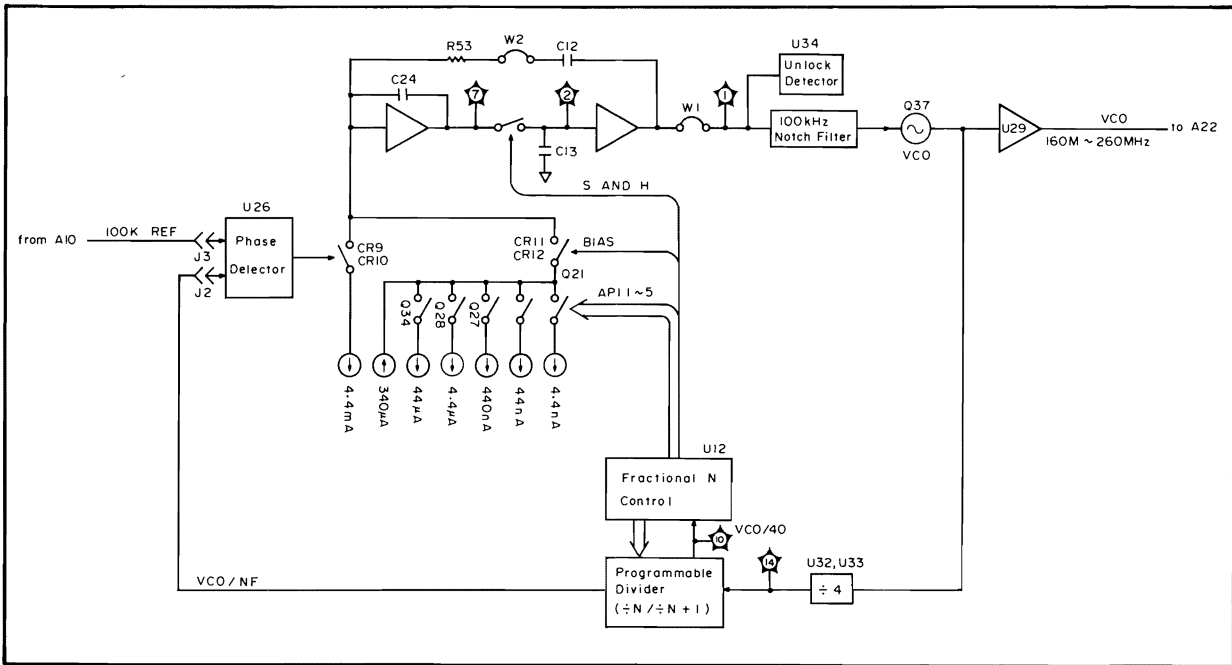
Figure A11-1. A11 Board Block Diagram
